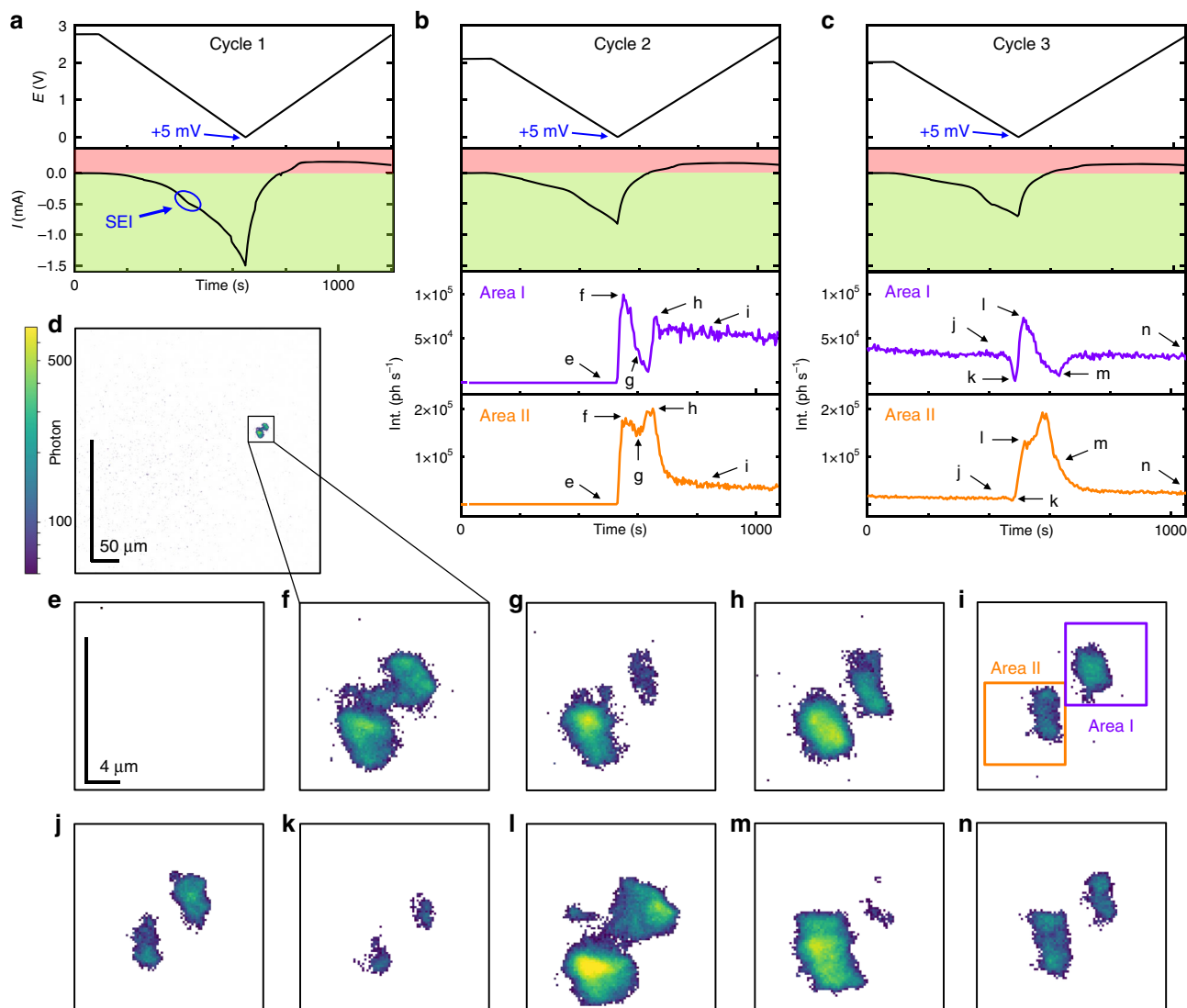
Fig. 2 Evolution of the early-stage defects from cycle 1 to 3. Potential (E) and current (I) of the 1st cycle (a). The E, I, and the integrated scattered intensity (Int) of the 2nd (b) and 3rd (c) cycle are shown separately for Area I and II. The light green and light red background in a–c illustrate the current for lithiation (negative currents) and delithiation (positive currents), respectively. d shows the complete FoV of 100 \times 430 \mu\text{m}^2 . e–n show the evolution of the observed defects at a higher magnification. The labels of e–n match the marked annotations in b and c, corresponding to the instants of time at which the FFDXM images were taken.
