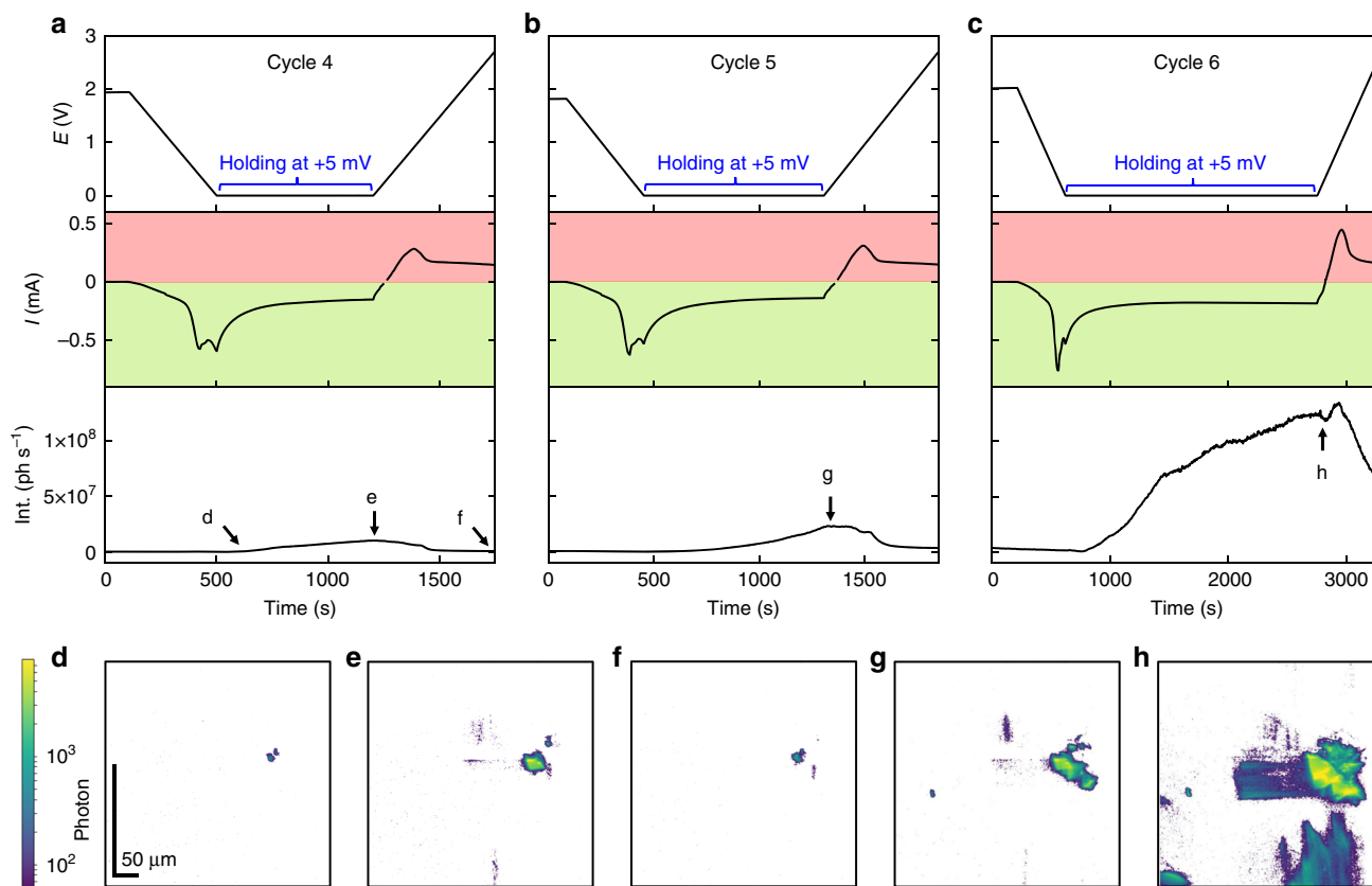
Fig. 4 Defect evolution from cycle 4 to 6. E , I , and Int curves of cycle 4 (a), 5 (b), and 6 (c). The light green and light red background illustrate the current range for lithiation (negative currents) and delithiation (positive currents), respectively. The labels of d-h match the marked annotations in a-c , corresponding to the instants of time at which the FFDXM images were taken.
