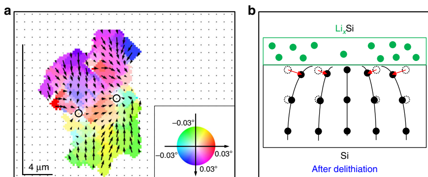
Fig. 3 Quantitative analysis of the early-stage defects. Result of 3D RSM (a). The direction and magnitude of the lattice tilt are expressed both by false colors (the reference color wheel is found in the inset) and arrows. The lattice tilt is the weakest at the center of the two defects, as indicated by the two circles in a. Cross-sectional schematic representation of the tilted lattice (b). The lattice is tilted toward the center of the defect, which is attributed to a lower lithium concentration in the defective area after delithiation.
