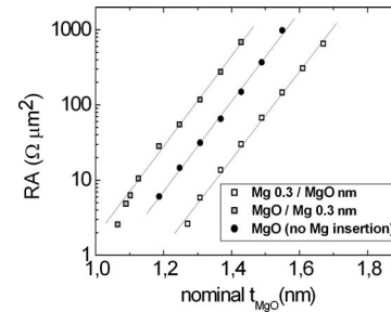
FIG. 2. RA product as a function of the as deposited MgO thickness for different 0.3 Mg insertions.
