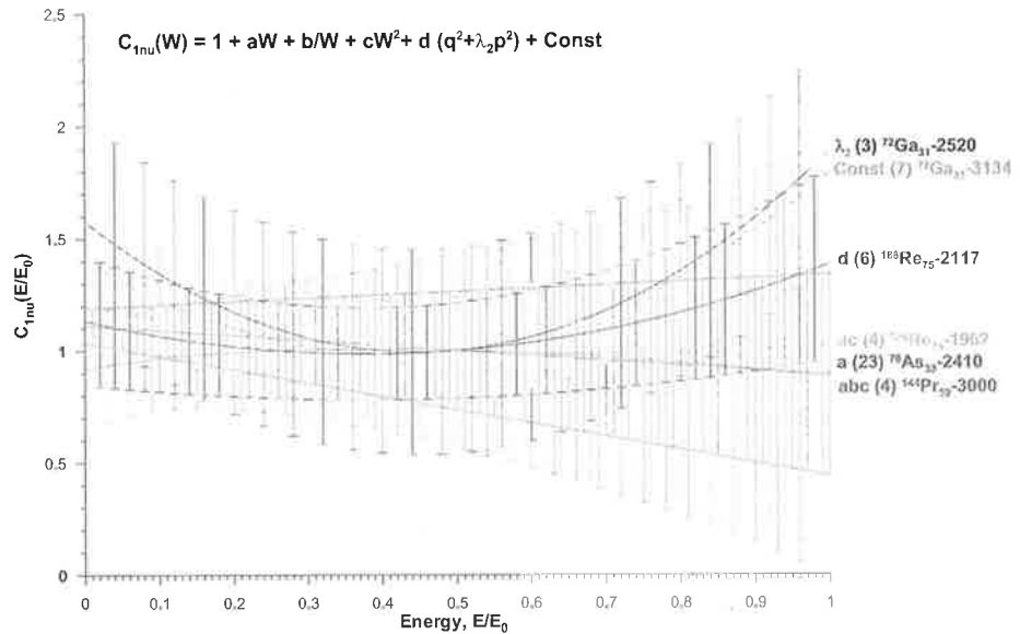
Figure 3 The spread of recommended 1nu shape factor curves for the analyzed experiments. Curves are normalized at a point that corresponds to the middle of the spectrum.
