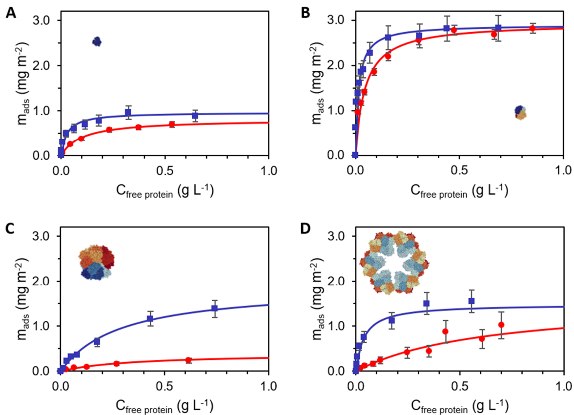
Figure 1. Adsorption isotherms of hemoproteins adsorbed on silica NPs: horse myoglobin (Mb) (A), pig hemoglobin (Hb) (B), Riftia pachyptila coelomic hemoglobin (HbC1) (C), Arenicola marina hemoglobin (HbAm) (D). Isotherms were performed in phosphate buffer ( 0.1 \text{ mol L}^{-1} ) pH 6 (blue squares) or pH 7 (red circles). For each condition, at least three replicas were done. The average values and standard deviations of the experimental points are shown. Data were fitted using the Langmuir adsorption model (solid lines) calculated on averaged data.
