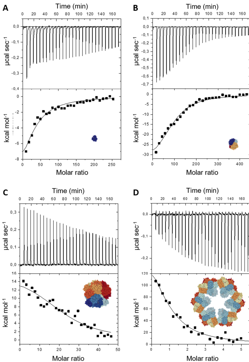
Figure 2. Isothermal titration calorimetry experiments of hemoproteins adsorbed on NPs in phosphate buffer ( 0.1 \text{ mol L}^{-1} , pH 7): horse myoglobin (Mb) (A), pig hemoglobin (Hb) (B), Riftia pachyptila coelomic hemoglobin (HbC1) (C), Arenicola marina hemoglobin (HbAm) (D). Upper
