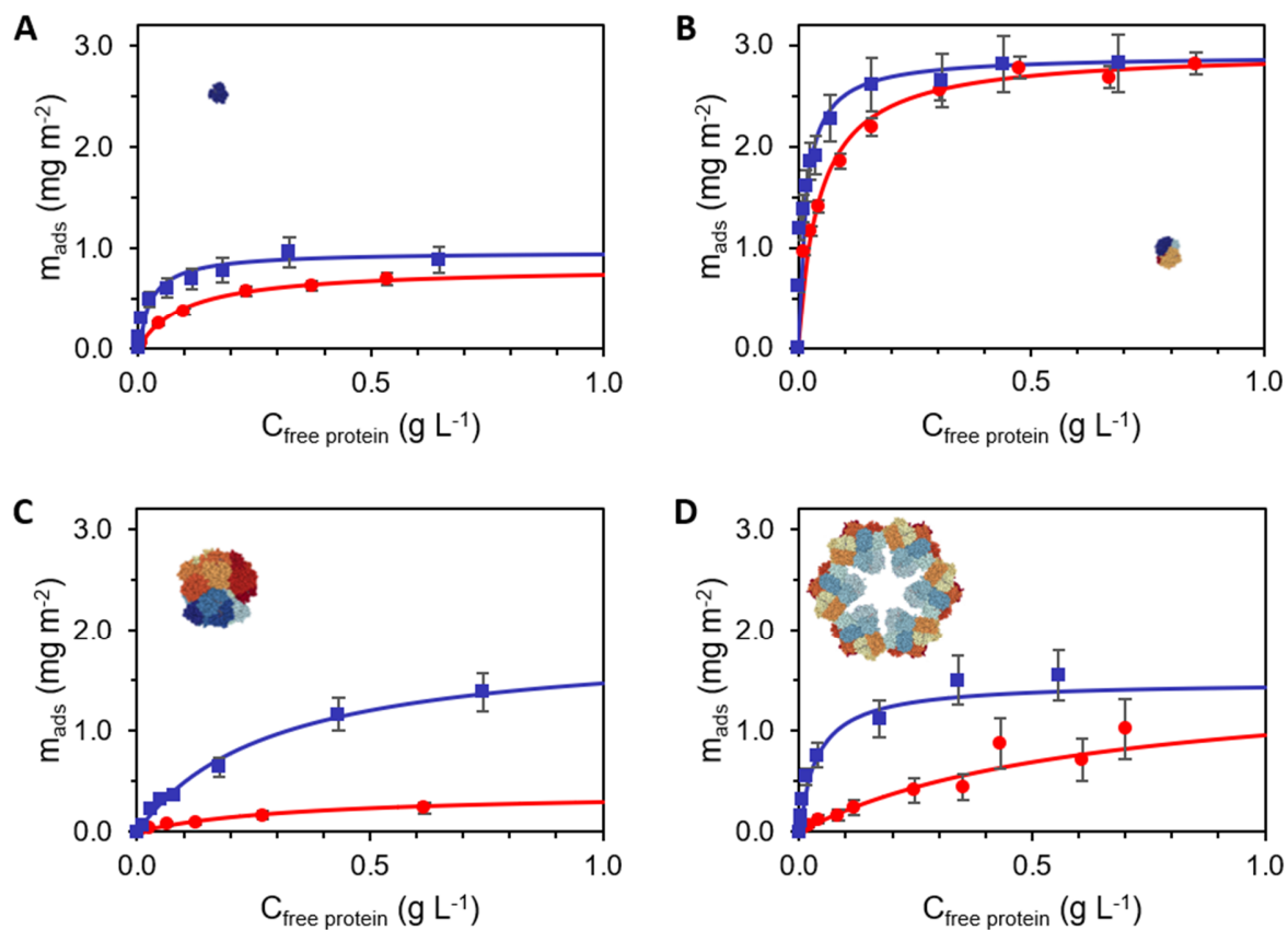
Figure 1. Adsorption isotherms of hemoproteins adsorbed on silica NPs: horse myoglobin (Mb) (A), pig hemoglobin (Hb) (B), Riftia pachyptila coelomic hemoglobin (HbC1) (C), Arenicola marina hemoglobin (HbAm) (D). Isotherms were performed in phosphate buffer ( 0.1 \text{ mol L}^{-1} ) pH 6 (blue squares) or pH 7 (red circles). For each condition, at least three replicas were done. The average values and standard deviations of the experimental points are shown. Data were fitted using the Langmuir adsorption model (solid lines) calculated on averaged data.
