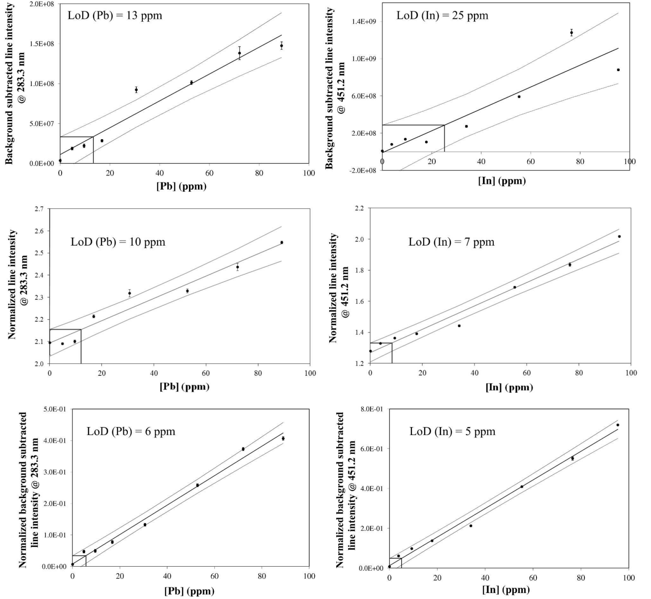
Figure 8: Calibration curves for the background-subtracted line intensity (top figures), the normalized raw intensity (middle figures) and normalized background-subtracted line intensity (bottom figures) of lead (left handside figures) and indium (right handside figures) in liquid sodium. Each point is the result of the accumulation of 4000 laser shots. The prediction bands are drawn for a 95% confidence level and are calculated from 10 replicas per concentration.
