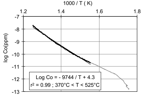
Fig. 3. Oxygen measurement after hydrogen ( \text{Ar} + 4\% \text{H}_2 specially prepared) reduction at 540\text{ }^{\circ}\text{C} in the BIP static facility where the chromium saturation is assumed and using the calibrated constants for the emf conversion from the oxygen sensor output ( r^2 being the linear regression coefficient).
