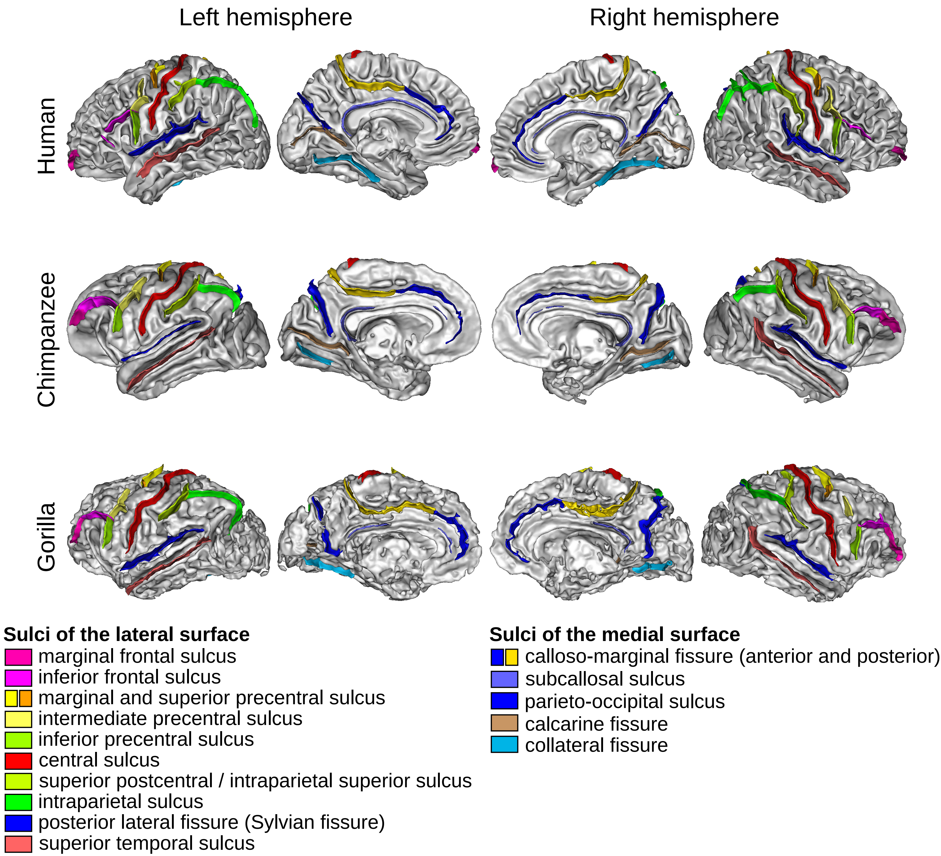
Figure 1: Each row shows the template that is used to represent one of the species. For each template the grey–white surface segmented by Morphologist is shown, as well as the sulci that were used in the interspecies registration.
