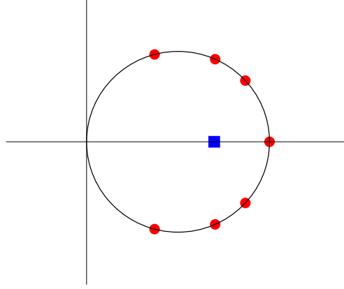
Figure 1. A sketch of the spectrum of the FDR matrix \mathbf{X} in a typical situation with N = 7 . Red circles: individual eigenvalues \tilde{X}_k . Blue square: their center of mass X_{\mathrm{typ}} .
