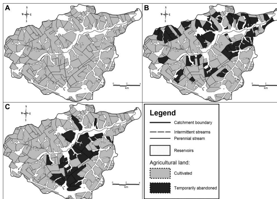
Fig. 2 Reconstruction of the area of cultivated and abandoned land in the River Lokna basin during the period 1990–2009: (A) no abandoned fields in 1990; (B) cultivated and abandoned fields in 2002 (from Landsat ETM satellite images); (C) cultivated and abandoned fields in 2009 (direct field observations).
