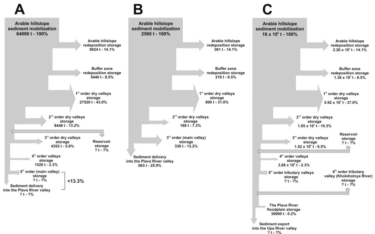
Fig. 4 Provisional sediment budgets: (A) and (B) annual budgets for the Lokna and Lyapunovka key sub-catchments respectively; (C) sediment budget for the entire River Plava basin for the period 1986–2009.
