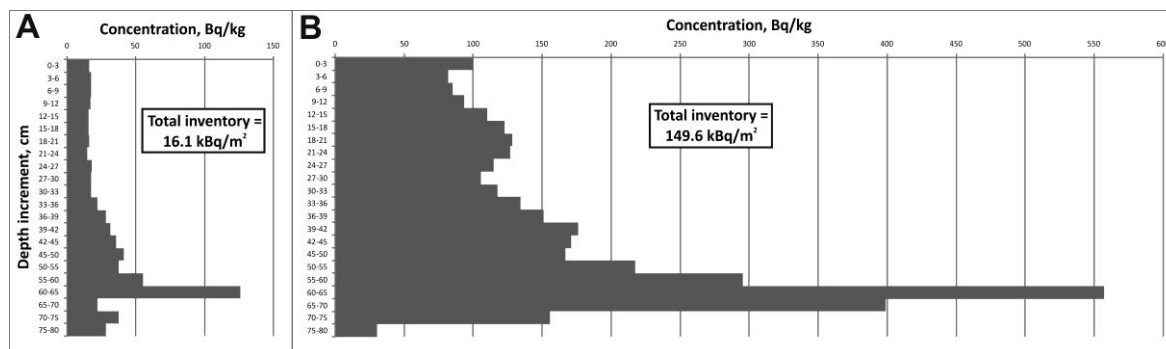
Fig. 5 The ^{137}\text{Cs} depth distribution curves (shown on the same X-axis scale to facilitate comparison) and inventories associated with the River Upa floodplain sediment upstream (A – section UP-2), and downstream (B – section UP-1) from the River Plava confluence. For precise section locations see Fig. 1(B).
