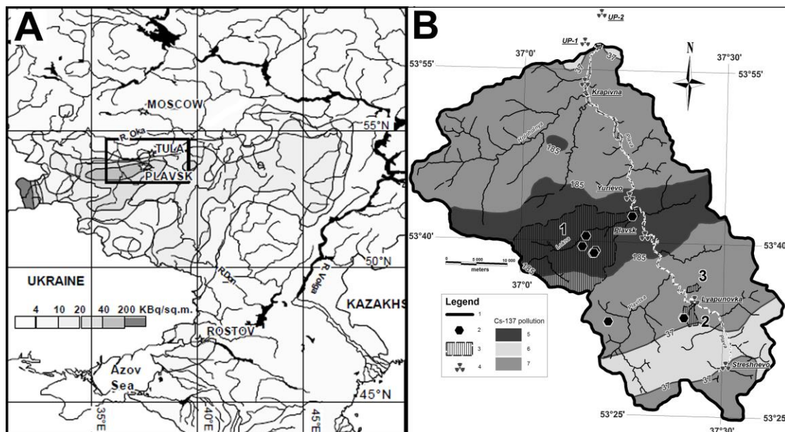
Fig. 1 (A) Location of the study area within European Russia and a generalized map of Chernobyl-derived 137 Cs contamination (based on Izrael, 1998). (B) Map of the River Plava basin showing the initial Chernobyl-derived fallout 137 Cs (based on Izrael, 1998) and the location of the study sites. Legend: 1) the River Plava basin boundary; 2) 137 Cs baseline fallout reference sampling sites; 3) the key sub-catchments (1 – the River Lokna; 2 – the Lyapunovka dry valley; 3 – the Sviatoy Istochnik dry valley); 4) the floodplain sampling sites. Levels of initial 137 Cs fallout: 5) <37 kBq m -2 ; 6) 37–185 kBq m -2 ; 7) >185 kBq m -2 .
