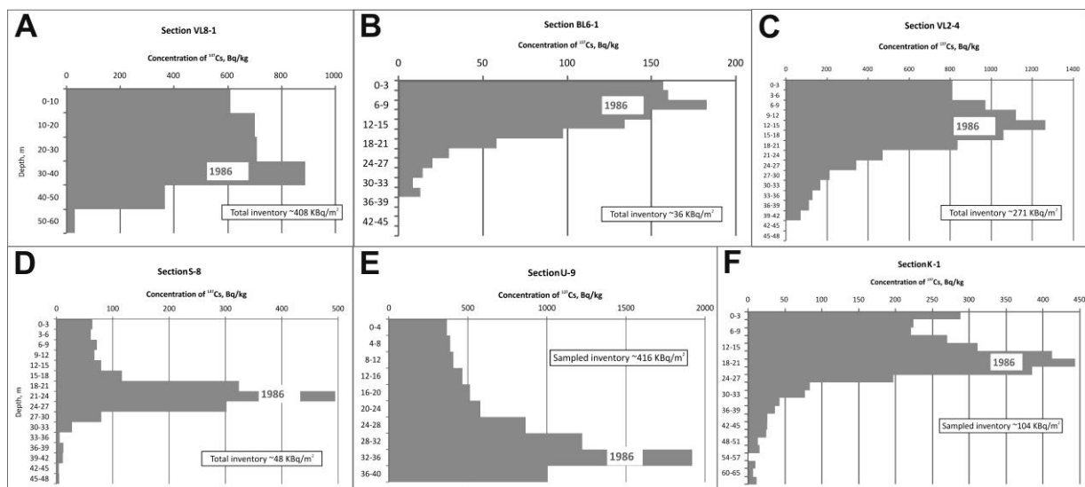
Fig. 3 Examples of typical ^{137}\text{Cs} depth distributions in sediment deposited in the bottoms of valleys of different orders: (A) Formerly cultivated head of the Upper Lokna dry valley tributary (1st order); (B) Transport reach of the Lyapunovka dry valley (2nd order); (C) the Upper Lokna dry valley (3rd order). The Plava River floodplain: (D) Streshnevo site (4–5th order transition); (E) Yurievo site (6th order); (F) Krapivna site (7th order).
