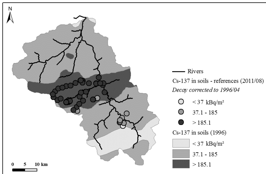
Fig. 4 A comparison of the point estimates of ^{137}\text{Cs} inventory derived from the field measurements using the model presented in Fig. 3 with the values depicted on the initial contamination map produced by Izrael et al. (1998). The estimates of ^{137}\text{Cs} inventory derived from the field measurements have been corrected for decay to be directly comparable with the data presented by Izrael et al. (1998) which relate to April 1996.
