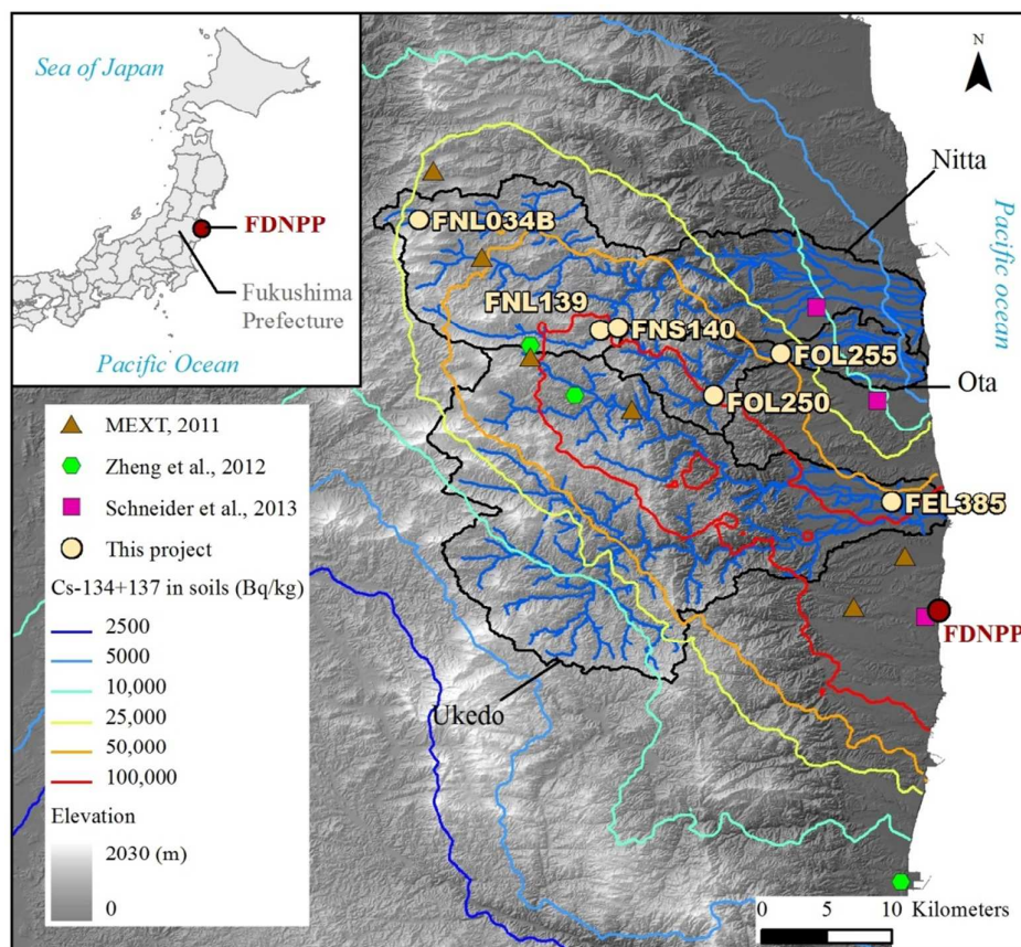
Figure 1. Location of the main inland radiocesium contamination plume in northeastern Japan (colored lines), the analyzed samples (white dots), and samples analyzed in other studies in which plutonium was detected (colored dots).
