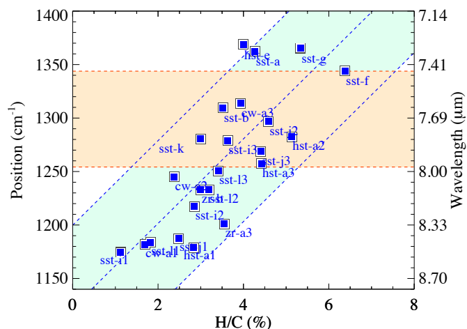
Fig. 11. Evolution of the “1300 \text{cm}^{-1} ” peak maximum position in analogue spectra displayed according to the elemental hydrogen to carbon ratio measured independently. The blue coloured region encloses the confidence interval of the correlation. The orange coloured region corresponds to the observed range for the astronomical observations analysed in this article.
