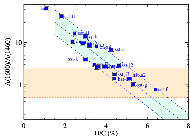
Fig. 10. Comparison between analogue spectra integrated-intensity ratios of aromatic C=C band at 1600\text{ cm}^{-1} , and aliphatic \text{CH}_x band at 1460\text{ cm}^{-1} as a function of the elemental hydrogen to carbon ratio measured independently. The blue coloured region encloses the confidence interval of the correlation. The orange coloured region corresponds to the observed range for astronomical observations.
