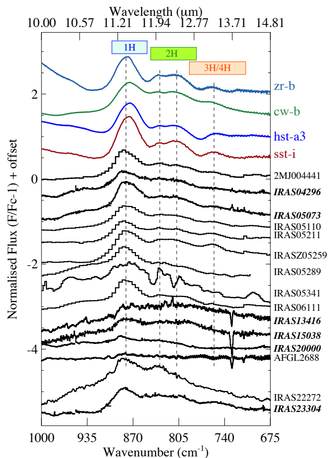
Fig. 8. Zoom on Spitzer and ISO spectra of class C and D type sources analysed in the out-of-plane aromatic CH mode's spectral region. The sources labelled in italics correspond to available Spitzer high-resolution spectra ( R \sim 600 ). Several analogues produced in different ball-milling environments are displayed above, for a direct comparison of the position of the observed bands and a range of measured relative intensities. The typical span of expected positions for the CH out of plane bands according to the underlying aromatic structure to which they are attached are given above (1H: solo; 2H: duo-bay, armchair; 3H: trio; 4H: quartet).
