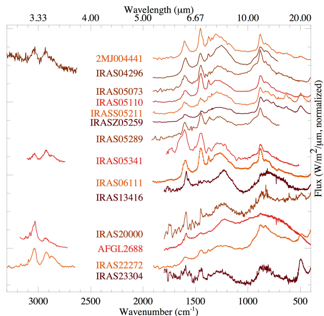
Fig. 1. Astronomical observations of class \mathcal{C} and \mathcal{D} sources, displaying characteristic infrared emission bands.
