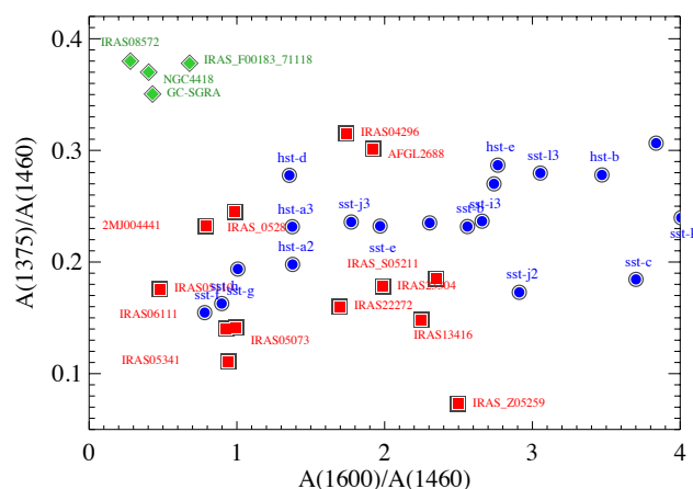
Fig. 9. Comparison between astronomical spectra integrated-intensity ratios of aromatic C=C band at 1600\text{ cm}^{-1} to aliphatic \text{CH}_x band at 1460\text{ cm}^{-1} according to the aliphatic \text{CH}_x 1375\text{ cm}^{-1}/1460\text{ cm}^{-1} ratio. The green diamonds correspond to the diffuse interstellar medium a-C:H absorptions. The red squares correspond to the class C and D sources in this study. The blue dots are the same ratios measured on the infrared spectra of the produced analogues.
