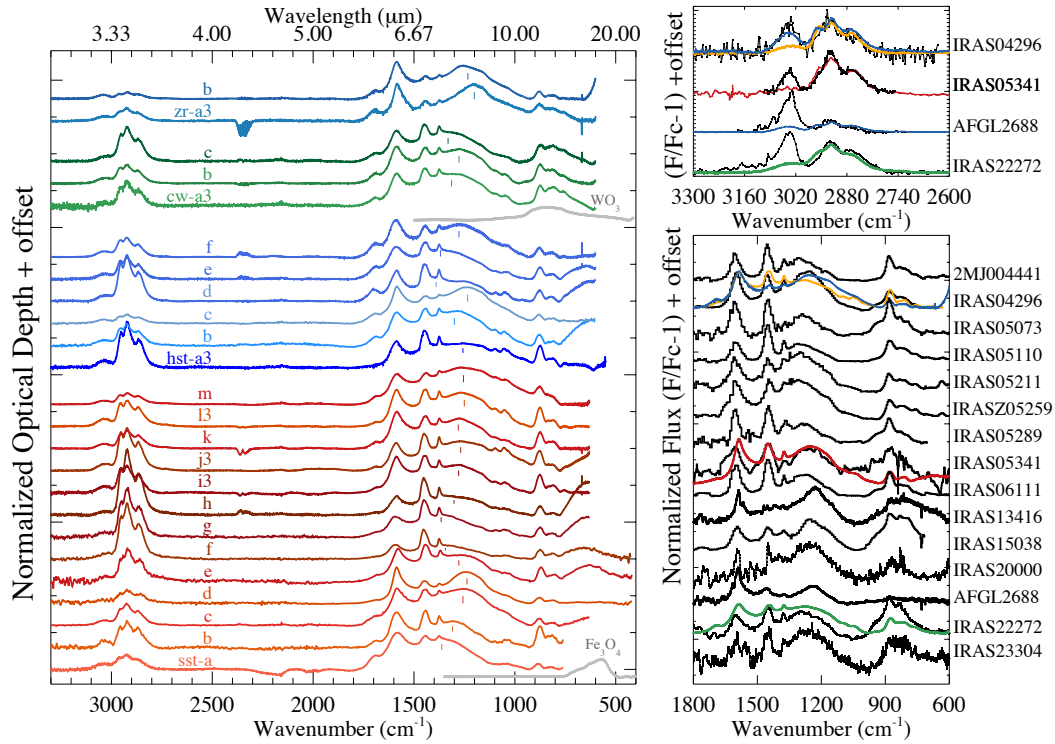
Fig. 6. Left panel: infrared spectra of the mechanochemically produced interstellar analogues, baseline subtracted. The colours correspond to different milling materials (stainless steel: red; hardened steel: blue; tungsten carbide: green; zirconium oxide: cyan). Infrared spectra of potential main contaminant for long-duration milling times are shown for clarity: iron oxide nanoparticles ( \text{Fe}_3\text{O}_4 spectrum from Can et al. 2010 ) for stainless steel and hardened steel and tungsten oxide ( \text{WO}_3 spectrum from Dawson et al. 2011 ), expected to be marginal due to its high shear resistance, for tungsten carbide. The thin lines indicate the estimated position of the peak maximum for the broad massif. The nomenclature refers to the description in Table 2. Right panels: astronomical observations for comparison to the analogue spectra. Top: near-infrared literature spectra available for four out of all the analysed sources. Bottom: mid-infrared Spitzer and ISO spectra of class C and D type sources analysed. For the spectra including both near and mir spectra, a combination of analogue spectra are overlaid for comparison.
