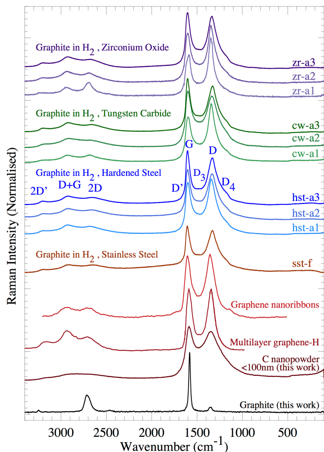
Fig. 5. Raman spectra of a sample set of planetary ball-milled graphite under a pressurised hydrogen atmosphere in function of milling time. The millings were performed in bowls made of stainless steel, hardened steel, tungsten carbide, and zirconium oxide. The Raman intensities were normalised. A graphite chunk and carbon nanopowder were measured for comparison. The spectra recorded for hydrogenated multilayer graphene (Ilyin et al. 2011) and graphene nanoribbons (Jovanović et al. 1996) are displayed.
