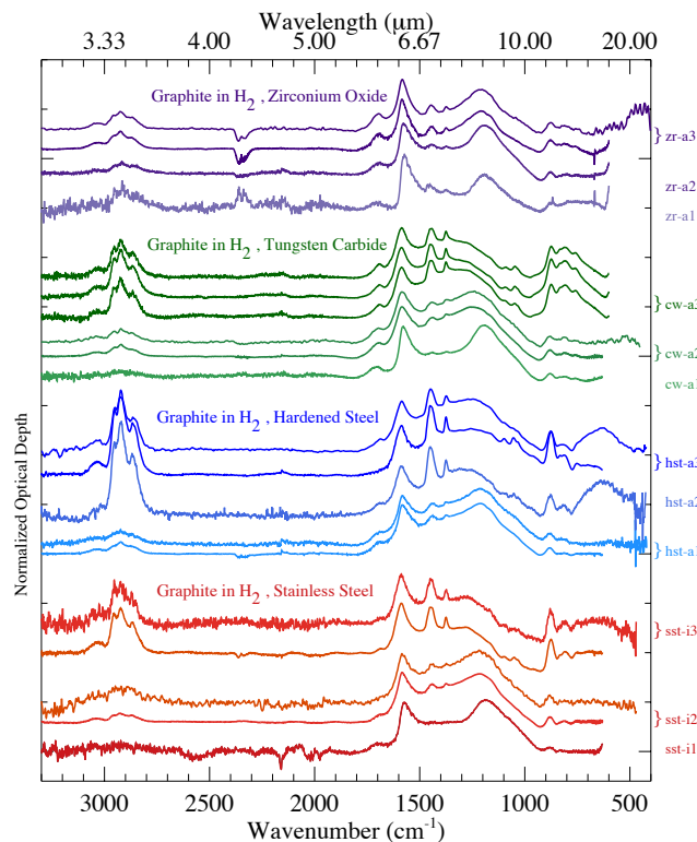
Fig. 3. Infrared spectra of a sample set of planetary ball-milled graphite under a pressurised hydrogen atmosphere in function of milling time. The millings were performed in bowls made of stainless steel, hardened steel, tungsten carbide, and zirconium oxide. The spectra were continuum subtracted.
