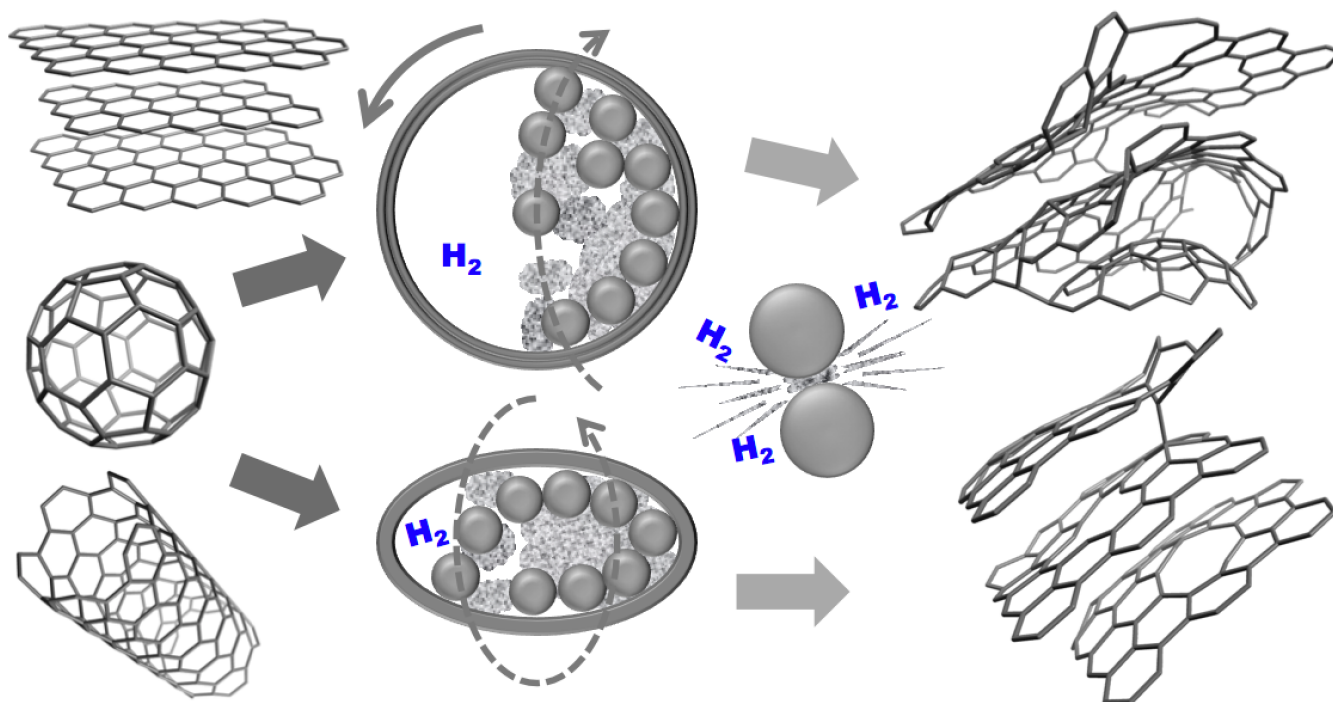
Fig. 2. Schematic representation of the top down mechanochemical process performed with a planetary ball mill (upper) and high-energy mill (lower). The milling impacts and shattering modify the size or crosslink graphite grains, flakes, carbon nanotubes and fullerenes down to the nanometre scale, and a defect-induced chemistry takes place in the pressurised hydrogen-reducing atmosphere.
