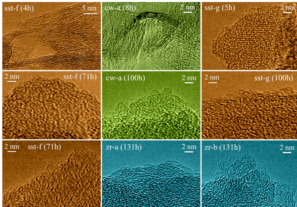
Fig. 7. High-resolution transmission electron microscope images for different ball-milled carbon precursors of this study and different mill materials. They are shown at large mechanochemical milling times performed in an hydrogen atmosphere. A few images are shown after a few hours of ball milling for comparison. The colour-coding for the images is brown for stainless steel, green for tungsten carbide, and light cyan for zirconium oxide experiments, respectively.
