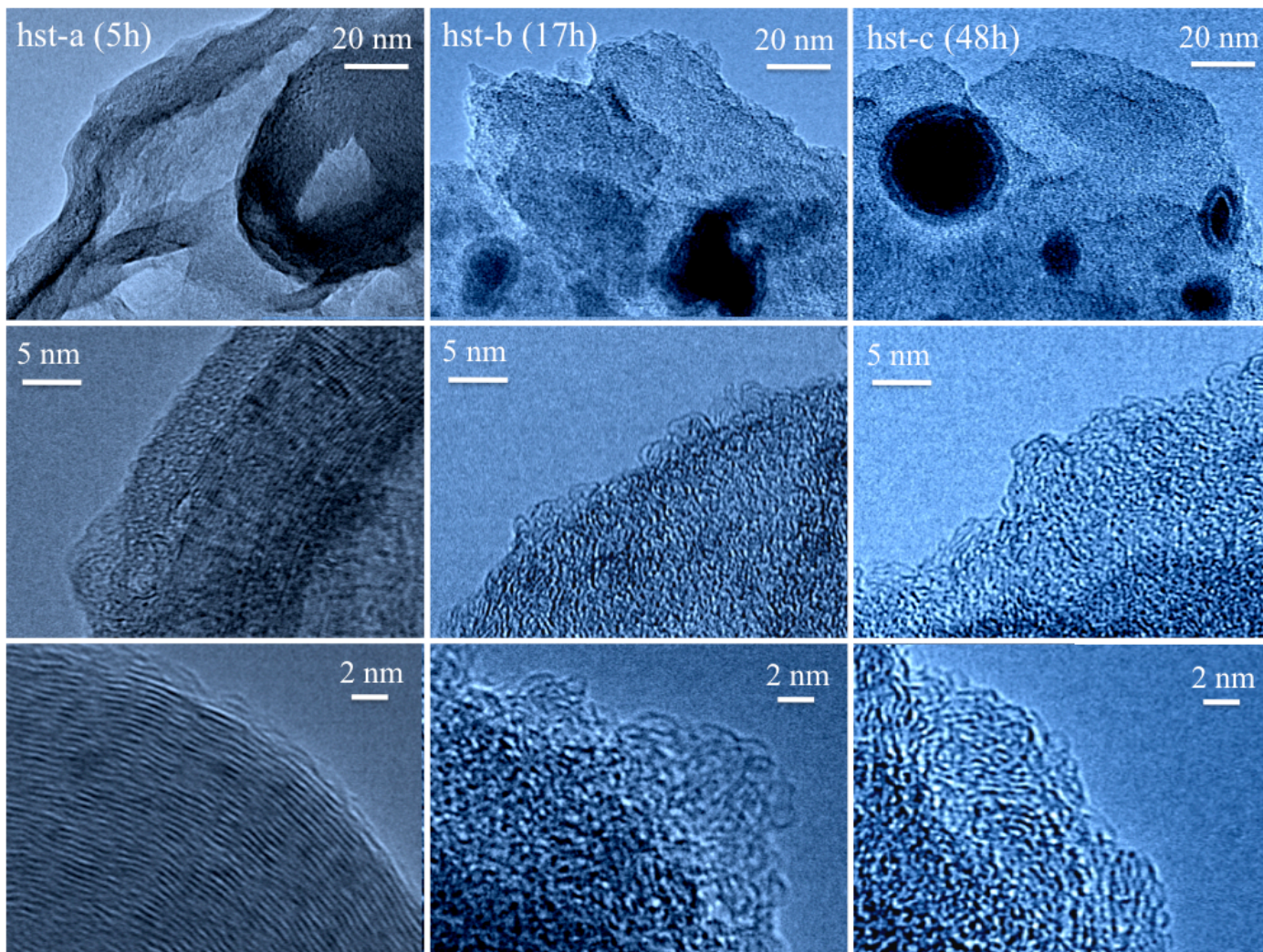
Fig. 4. High-resolution transmission electron microscope images at increasing magnification scales showing the structural evolution of ball-milled graphite under hydrogen atmosphere for the hardened steel experiment in a planetary ball mill after 5 h ( left panels ), 17 h ( middle panels ) and 48 h ( right panels ). The ordered graphitic plane evolves rapidly toward a turbostratic structure, and, at high milling times, a fully disordered carbon network with a high curvature. We note the progressive contamination of the hydrogenated carbon structure by iron nanoparticles issued from the shattering of the bowl during the milling process, giving rise to dispersed isolated passivated iron nanoparticles.
