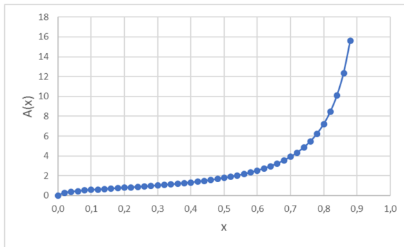
Figure 4: A function
