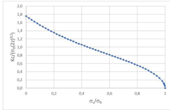
Figure 10: Critical stress evaluation from fracture stress
