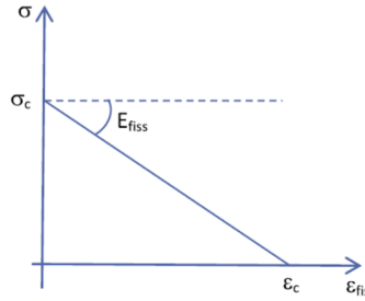
Figure 2: Smeared crack model
