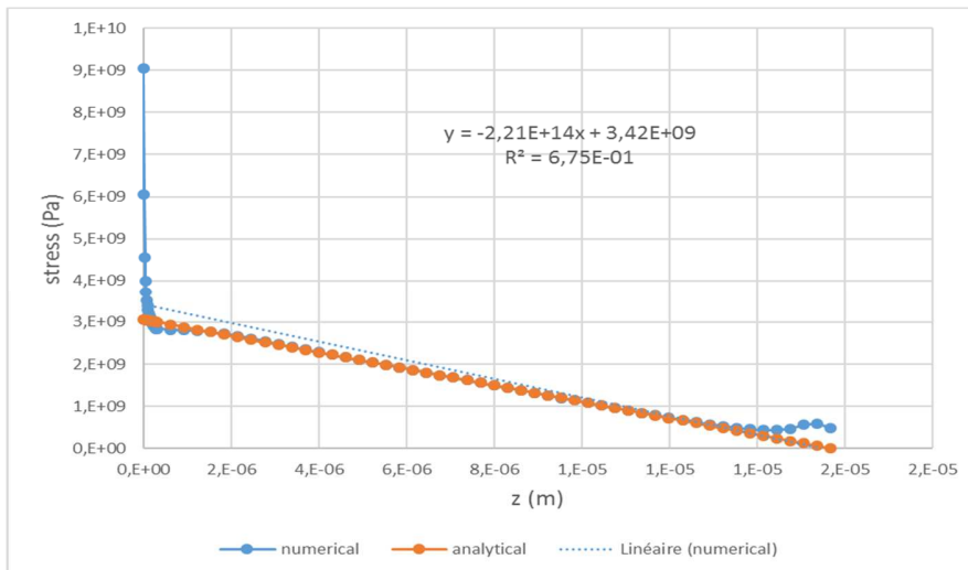
Figure 11: Stress evolution along the length of the sample
