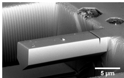
Figure 7: SEM image - Microscopic notched cantilever of fresh \text{UO}_2
