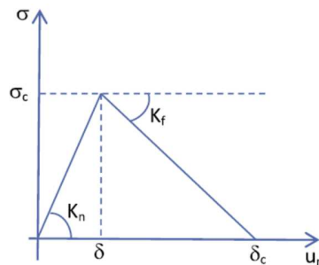
Figure 1: Stress versus displacement (crack opening) of the cohesive zone model
