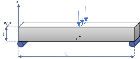
Figure 3: Three points bending sample
