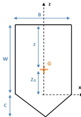
Figure 8: Notations for microscopic sample (pentagonal section)
