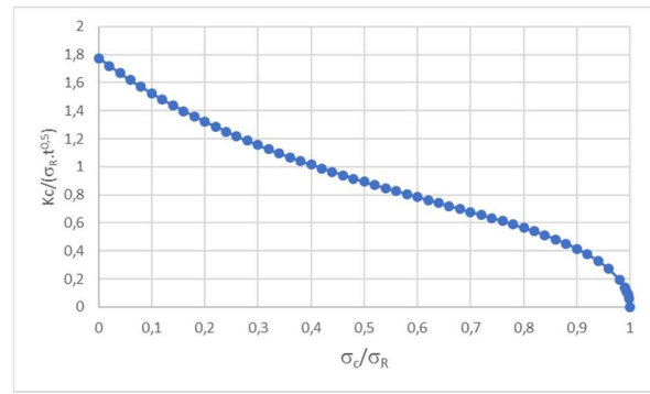
Figure 5: Critical stress evaluation from fracture stress
