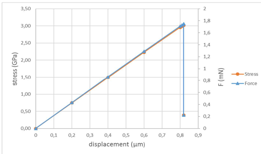
Figure 17: Stress and force versus displacement
