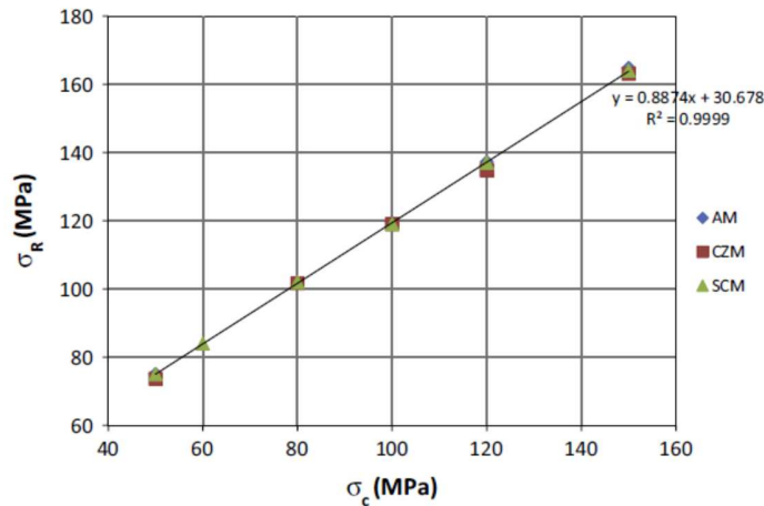
Figure 6: Comparison of the three approaches: Cohesive Zone Model, Smearred Crack Model and Analytical Model (respectively CZM, SCM and AM).
