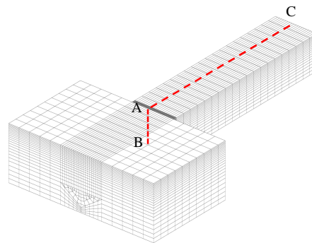
Figure 13 Meshing of the structure
