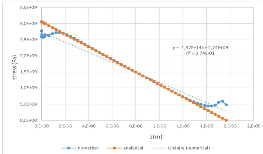
Figure 12: Stress evolution along the length of the sample
