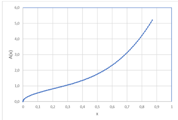
Figure 9: A function
