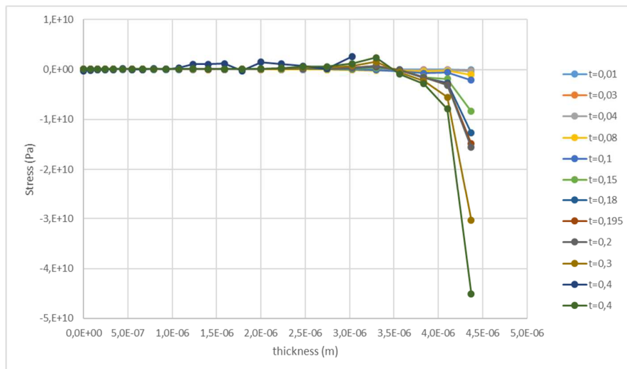
Figure 15 Stress evolution along the thickness of the beam
