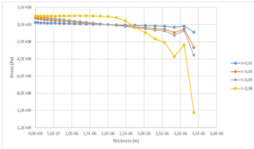
Figure 14 Stress evolution along the thickness of the beam
