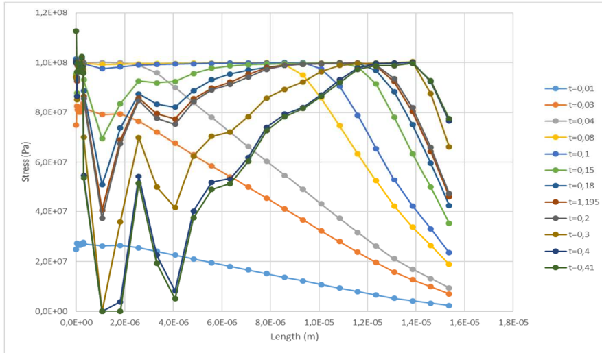
Figure 16 Stress evolution along the length of the beam
