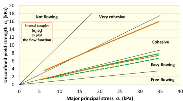
Fig. 4. Flow functions and bulk level cohesion (Ref. 8)
