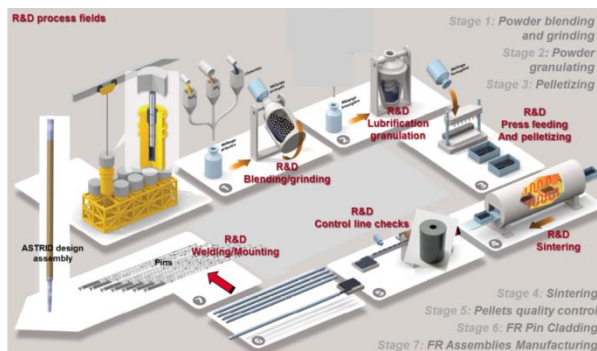
Fig. 1. SFR fuel fabrication process at a glance
