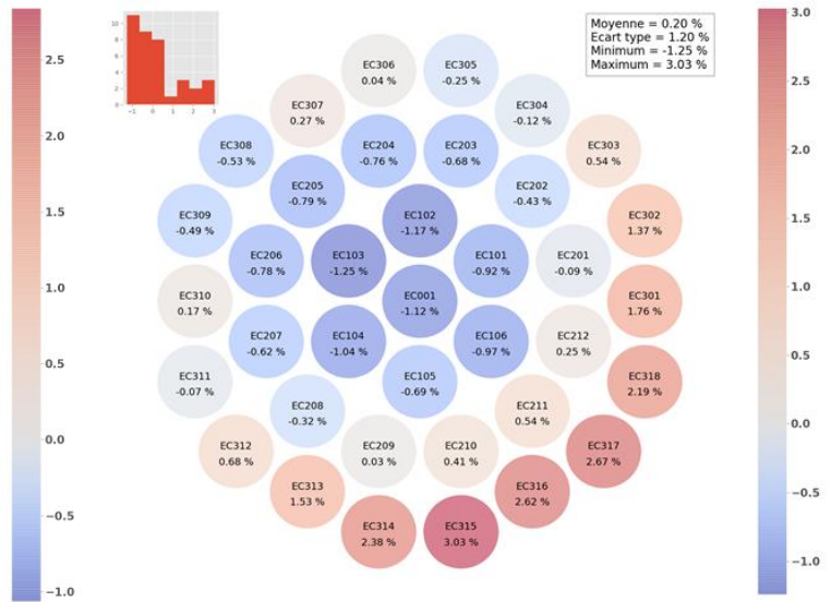
Figure 8. AP3-TR4 Bias on Fission Rates per Assembly new APOLLO3® Scheme.
