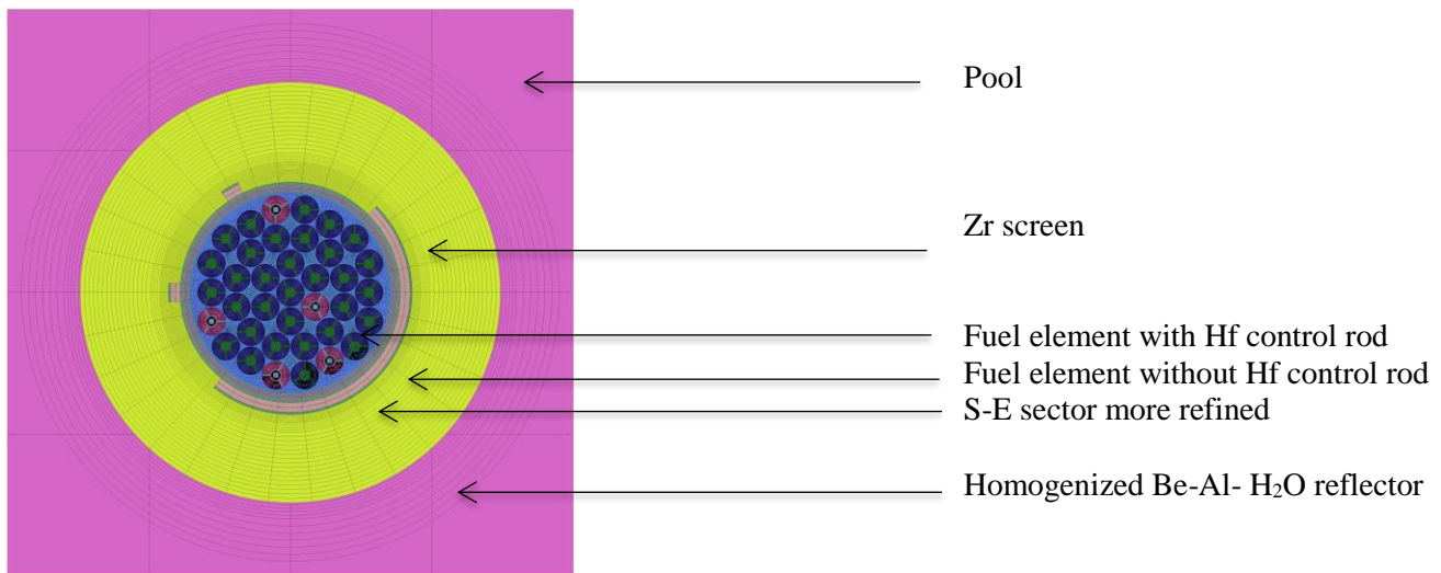
Figure 5. Meshed Core Geometry for New APOLLO3 ® Scheme.
