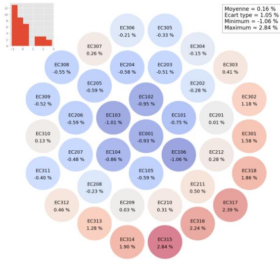
Figure 7. AP3-TR4 Bias on Fission Rates per Assembly iso-HORUS3D/N Scheme.
