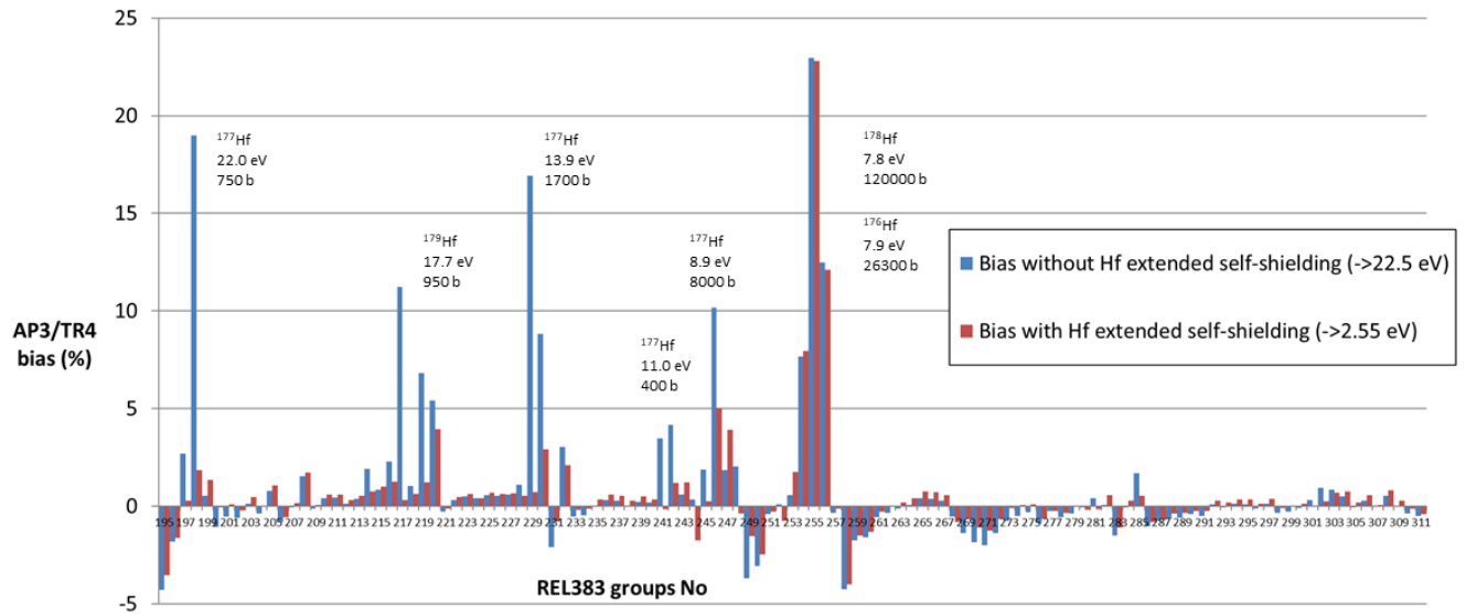
Figure 6. AP3/TR4 Absorption rate Bias in Hf
