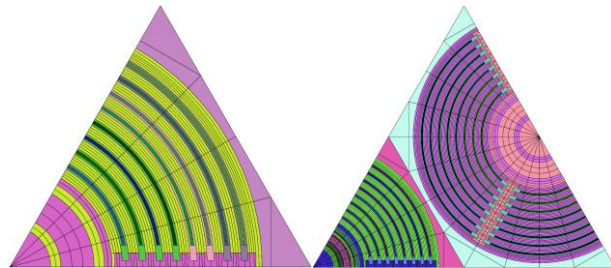
Figure 4. New Scheme Without/With Hf Lattice Geometry.
