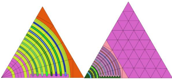
Figure 3. Iso-HORUS3D/N Without/With Hf Lattice Geometry.
