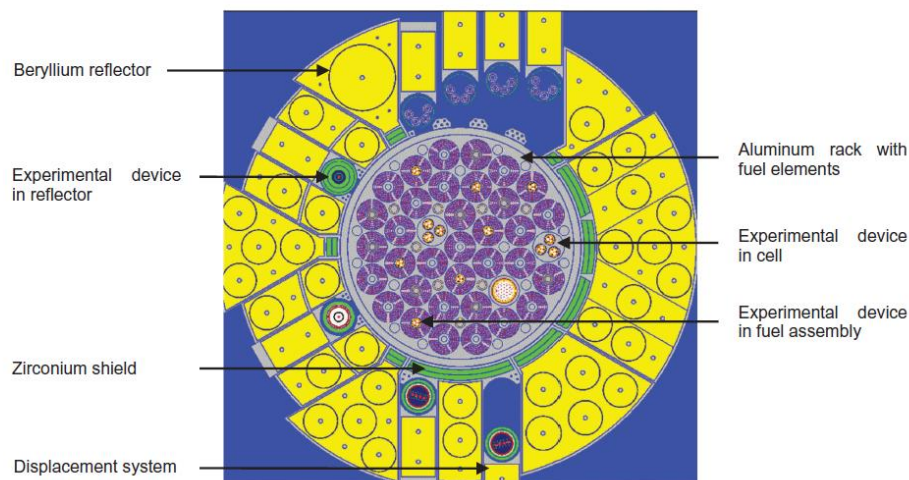
Figure 1. JHR Core Description
