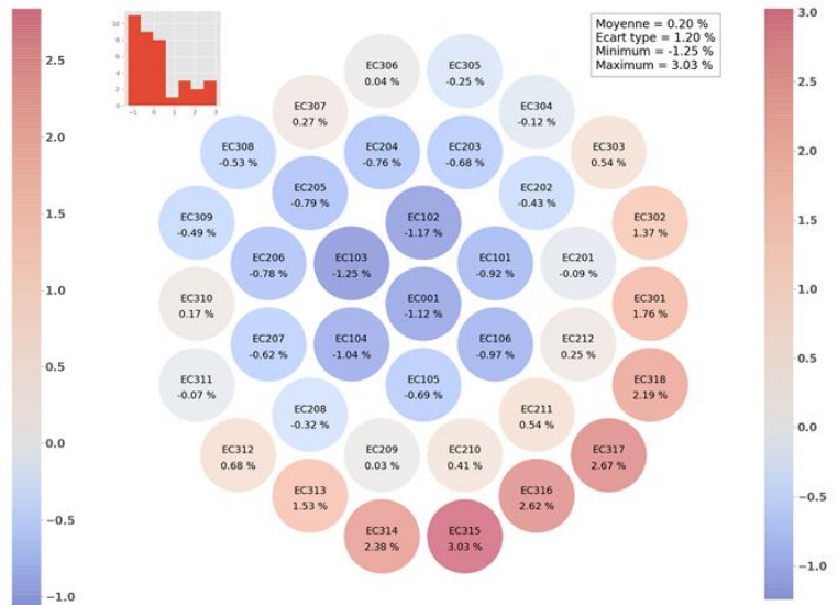
Figure 8. AP3-TR4 Bias on Fission Rates per Assembly new APOLLO3® Scheme.
