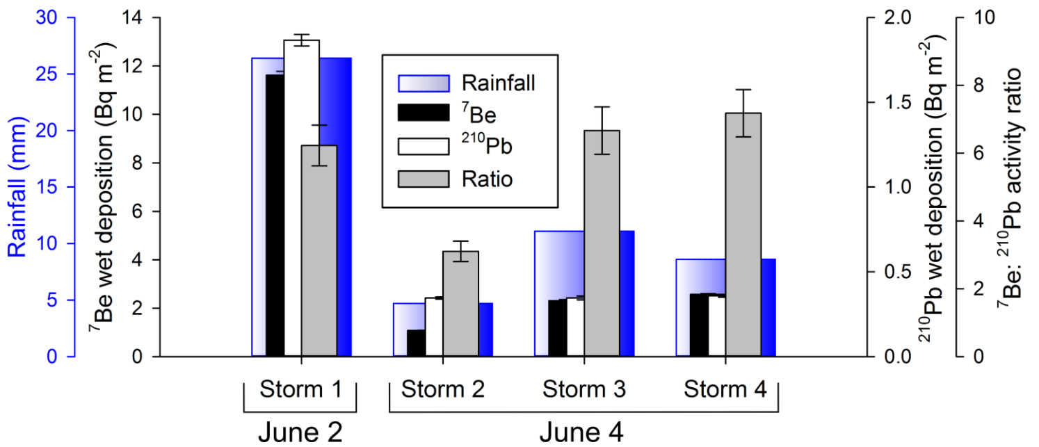
Fig. 6: Temporal variability of radionuclide deposition storm by storm at S10 (from June 2 to 4): cumulated rainfall (mm), cumulated ^{7}\text{Be} and ^{210}\text{Pb} deposition ( \text{Bq m}^{-2} ) and ^{7}\text{Be}: ^{210}\text{Pb} ratio. Error bars represent 1\sigma uncertainty.
