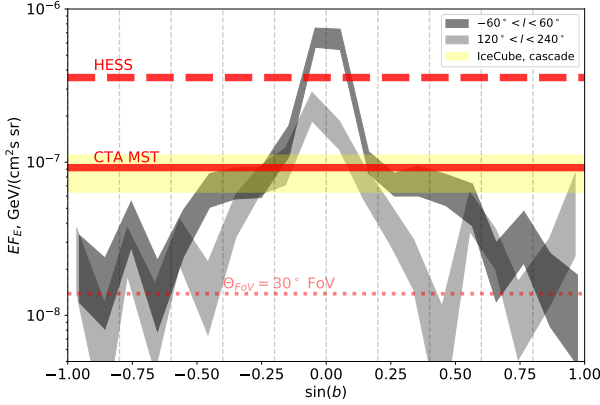
Fig. 4. Sensitivities of HESS, CTA/MST and a hypothetical 30° FoV IACT system for measurements of the Galactic latitude profiles of diffuse emission (100 h exposures per bin, each of \Delta \sin(b) = 0.1 in width, 1000 h total exposure) at 30 TeV reference energy. Yellow horizontal shading shows the level of the astrophysical neutrino flux measured by IceCube in cascade mode (Williams 2019). Light and dark grey shaded bands show an extrapolation of the Fermi /LAT measurements at 1 TeV, assuming the spectral slope \Gamma_\gamma = 2.4 (Neronov & Semikoz 2020).
