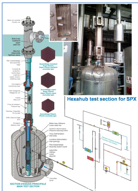
Fig. 7: Sketch and picture of the BACCARA facility
