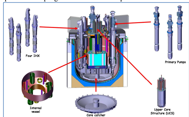
Fig. 1: Cut view of the ASTRID Primary circuit
