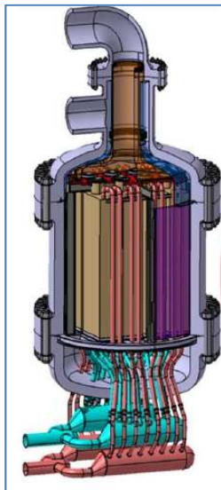
Fig. 8: Sketch of a SGHE module
