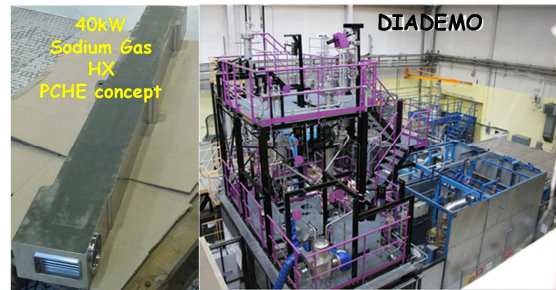
Fig. 9: Picture of the sodium gas PCHE mockup and DIADEMO facility where the HX mockup are tested
