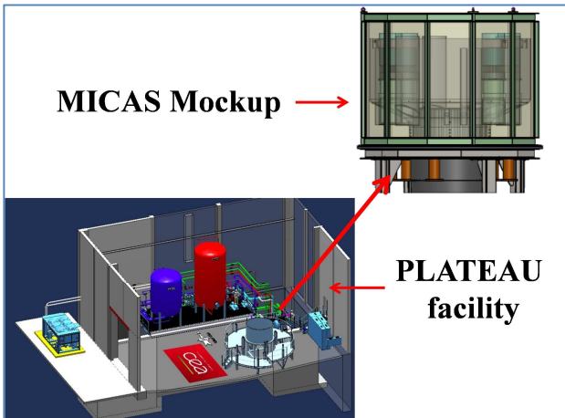
Fig. 6: Sketch of the PLATEAU facility and MICAS Mockup
