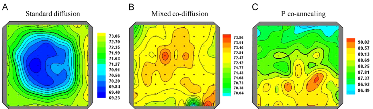
Fig. 3. Emitter R_{sheet} mappings. 4-point probe measurement on textured 156 psq wafers.
