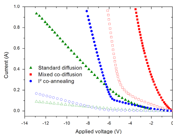
Fig. 7. Reverse dark current–voltage characteristics in linear drawing, measured before (filled symbols) and after (open symbols) cell edges removal by laser ablation. Cells surface moves from 239\text{ cm}^2 to 229.4\text{ cm}^2 .
