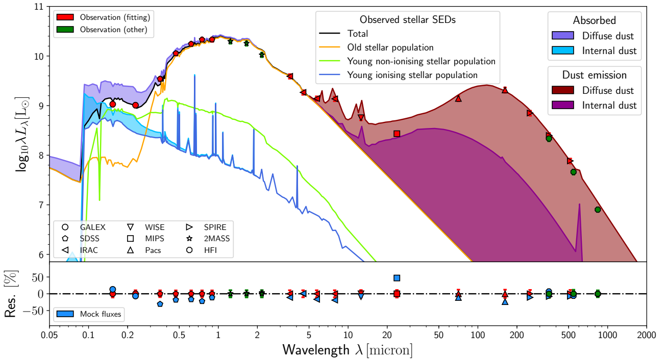
Fig. 6. Top panel: panchromatic SED corresponding to the SKIRT radiative transfer model for M81. The total observed stellar energy output is indicated with a black line and the total dust emission, when added to the stellar spectrum, follows the red line. The area shaded in purple above the observed stellar spectrum represents the radiation that is absorbed by the diffuse dust, thus the purple line represents the intrinsic stellar spectrum. Yellow, green, and dark blue lines represent the contribution of the old, the young non-ionising, and the young ionising stellar populations to the observed stellar spectrum, respectively. The area shaded in light blue above the young ionising population curve indicates the absorbed energy by internal (subgrid) dust. The area shaded in magenta between 20 and 500 \mu\text{m} indicates the energy distribution emitted by this internal dust. Bottom panel: comparison between the observed fluxes and the simulated SED, as relative residuals with the observations as reference. Observed fluxes are shown as red and green points, depending whether or not they were used in the fitting procedure. The blue points show the mock fluxes derived from the simulated SED.
