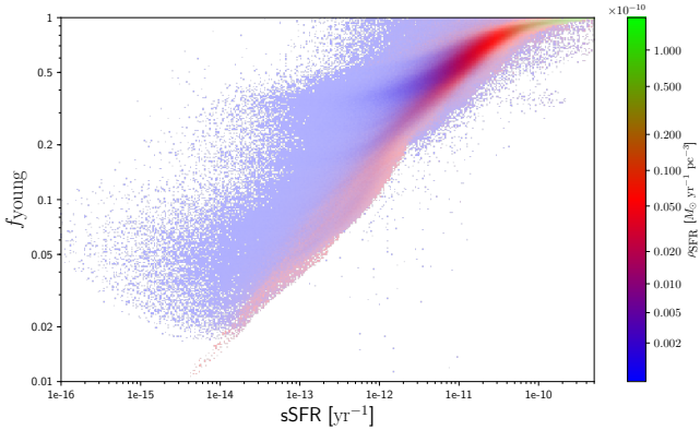
Fig. 13. Correlation between the specific star-formation rate and f_{\text{young}} , with the colour scale indicating the star-formation rate density, and the density of points represented by a transparency level.
