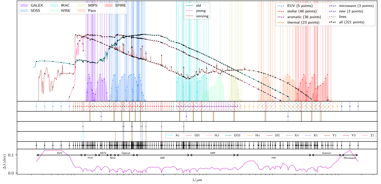
Fig. B.1. Wavelength grid used for the RT simulations. Top panel: 3 different stellar template spectra used for the models, on an arbitrary scale and normalised independently to match the frame. Rendered on top of these curves are black dots that show the points of the wavelength grid, to illustrate how they sample the intrinsic spectra of our model components. Also shown are the transmission curves of the filters for which we have observed data and for which we create mock observations. The coloured vertical lines plotted on top of these response curves show the additional sampling that is performed for each band, also shown as dots. Second panel: sampling of the different regimes with different densities, in a different colour per regime. The grid points with dashed vertical lines, and crossed out with the diagonal pattern, are removed and replaced by the wavelengths added for the sampling of the above filter response curve, because the number of points within the filter range was not sufficient. Third panel: wavelength grid points that have been placed at the effective wavelengths of the different bands. When this wavelength is close to an existing wavelength point, it replaces the original one (red and green lines), otherwise it is added as an additional wavelength (blue line and dot). Fourth panel: extra sampling that has been performed for prominent absorption and emission line features in the stellar spectra, adding a grid point at the peak (or valley) of the feature and at its edges. The position and origin of the corresponding line features are indicated in the fifth panel . The resulting wavelength grid is shown in the sixth panel . The density of the total grid in logarithmic space is plotted in the bottom panel , showing that the distance between any subsequent wavelengths in the grid is well below 0.05 dex, except in the EUV where the stellar emission is insignificant.
