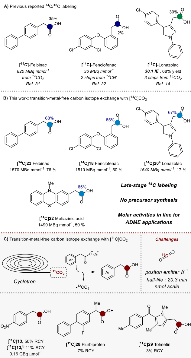
Scheme 4: Transition-metal-free CIE ^{14}\text{C} - and ^{11}\text{C} -labeling of pharmaceuticals. A) Methods previously reported. B) CIE with [ ^{14}\text{C} ]CO 2 . Molar activities for ^{14}\text{C} in MBq mmol -1 . C) CIE with [ ^{11}\text{C} ]CO 2 . Molar activities for ^{11}\text{C} in GBq \mu\text{mol}^{-1} . a Potassium salt prepared in situ and reaction performed out of the glovebox. b Preparative run, isolated yield.
