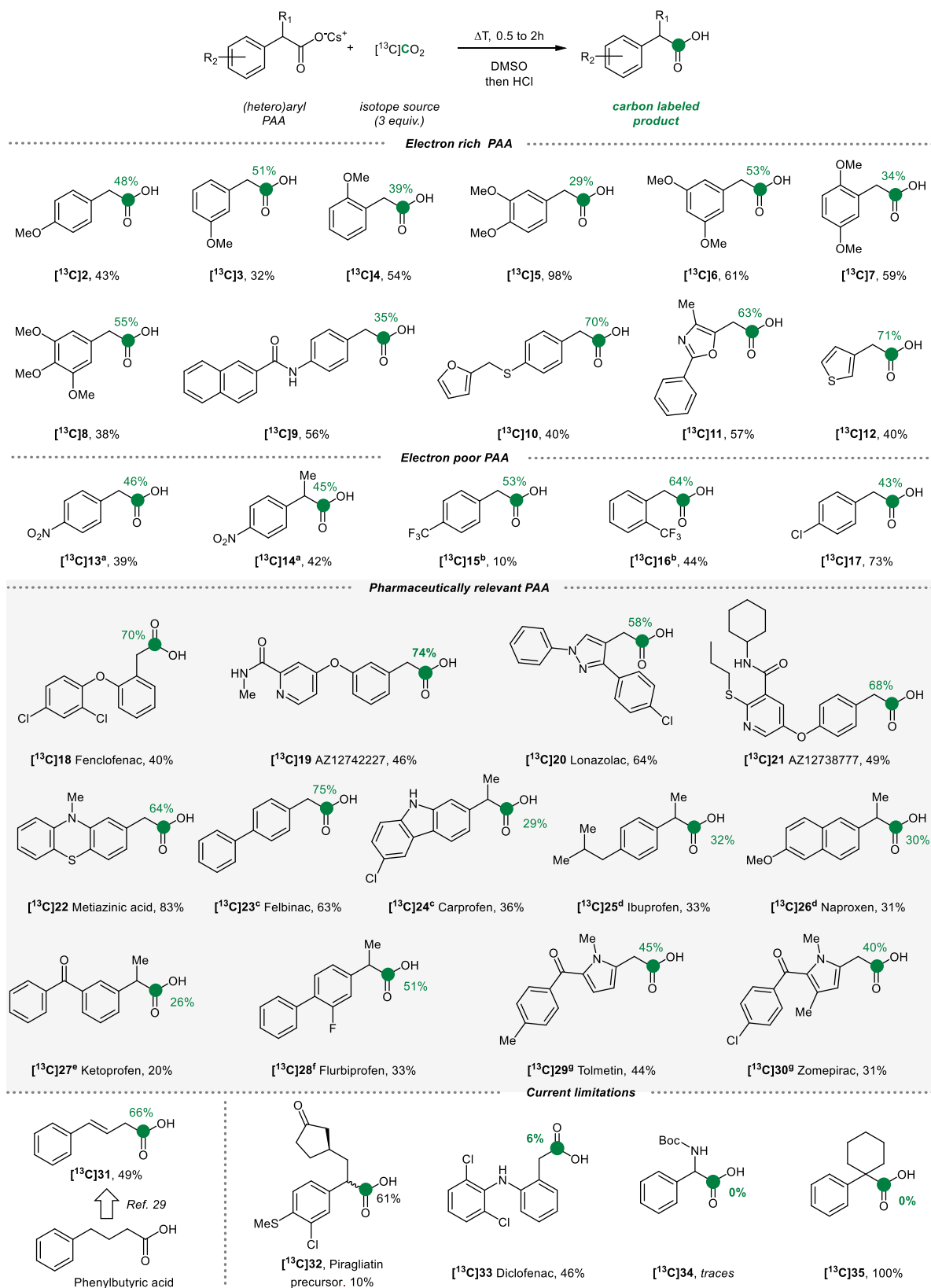
Scheme 3: 13 C-labeling of PAA. The green colored circles and numbers denote the positions of the atoms labeled and the percent incorporation of the isotope. Reaction conditions: substrate (0.1 mmol, 1 equiv.), 13 CO 2 (3 equiv.), DMSO (0.5 mL), temperature 150 °C, time 2 h. DMSO, dimethyl sulfoxide. a Reaction time 5 minutes, temperature 80 °C. b Reaction time 1h, temperature 130 °C. c Reaction time 4h. d Reaction time 6h, temperature 190 °C. e Reaction time 3.5h, temperature 190 °C. f Reaction time 0.5h, temperature 190 °C. g Reaction time: 5 minutes.
