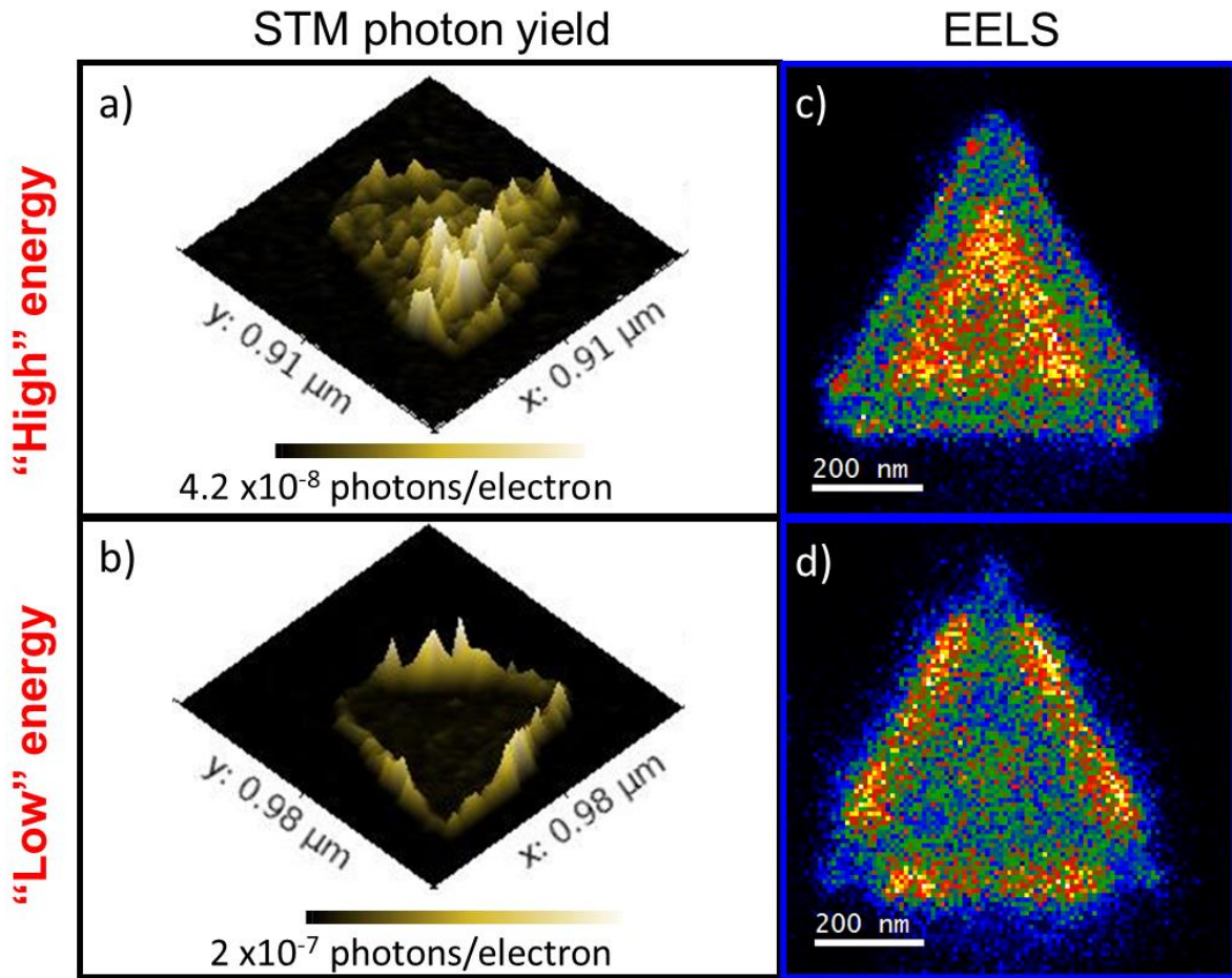
Figure 3: STM-excitation photon yield maps and EELS measurements (a)-(b) These photon yield maps are obtained by dividing the simultaneously acquired photon images by their corresponding current maps (see Section 2 in the Supporting Information for details). The result is thus an efficiency in terms of the number of photons emitted per tunneling electron. In other words, from these results we can predict the best location for the excitation in order to get the most emission at the desired wavelength. In (a), a 750/40 nm bandpass filter is placed before the detector, while in (b), photons in the range 900 \pm 20 nm are collected. The result is noticeably different for these two wavelength ranges. (c)-(d) Electron energy loss results. A high energy electron beam scans the particle and the energy lost by the electrons passing through the sample is measured. In (c) the number of electrons having lost energy in the 1.5-1.8 eV range as a function of e-beam position is plotted while in (d) the energy loss range is 1.1-1.4 eV. These results match the STM-excitation images qualitatively. The triangle side length is L \sim 630 nm.
