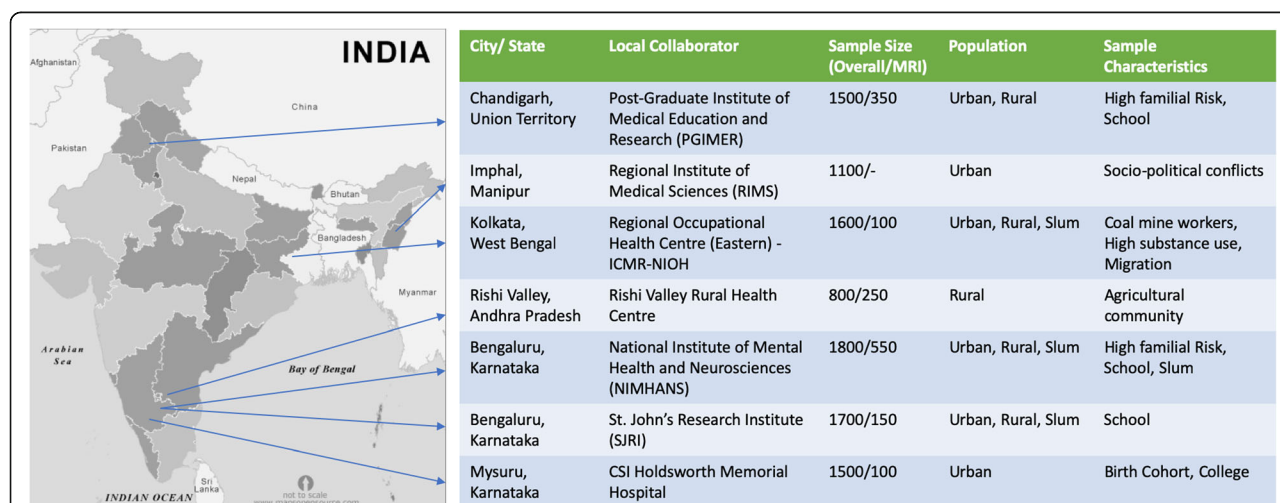
Fig. 4 cVEDA sample distribution and recruitment site characteristics (Map of India source: http://mapsopensource.com/india-states-outline-map-black-and-white.html ; As stated on the webpage "All the content by www.mapsopensource.com is licensed under a Creative Commons Attribution 3.0 Unported License")
