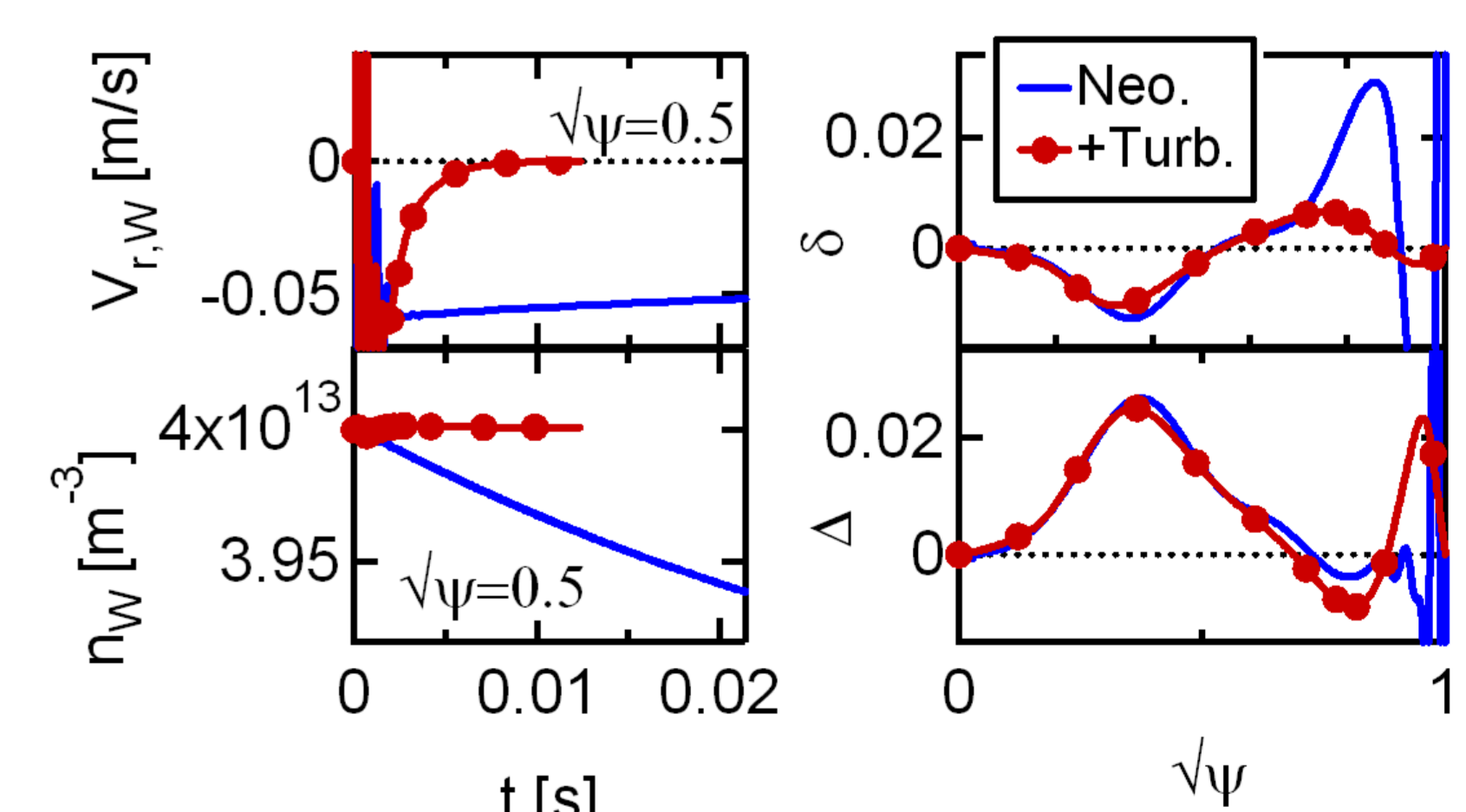
Fig. 10 : Radial flow & W^{28+} density at \nu_p = 0.5 (left); asymmetry profiles with and without turbulence (right).
