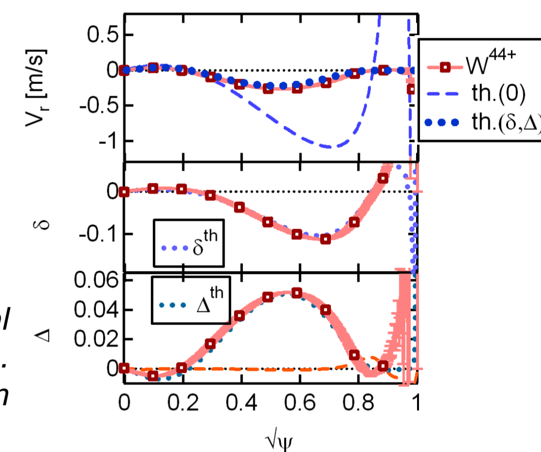
Fig. 6 : Radial flow, \delta and \Delta profiles for the real collisionality (peaked ion density profile). Comparison of simulation results with theory with (th(\delta, \Delta)) and without (th(0)) poloidal asymmetry.
