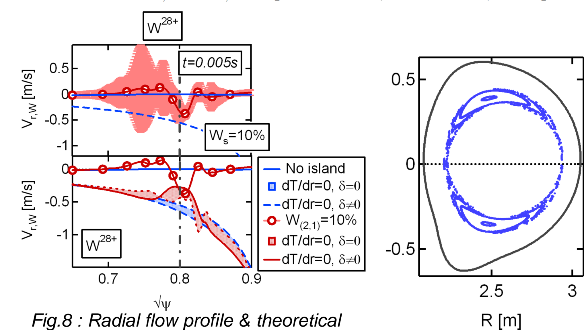
Fig. 8 : Radial flow profile & theoretical flow without thermal screening
