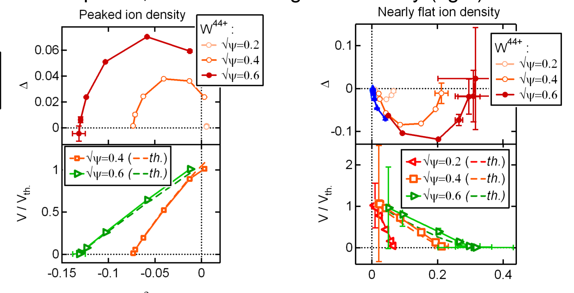
Fig. 5 : Asymmetry (top) and ratio of radial flow to theoretical value without asymmetry (bottom), for the peaked and flat ion density profiles, and several radial positions.
