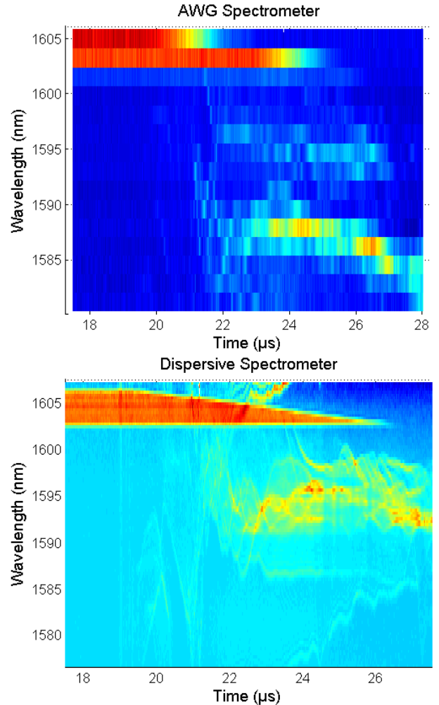
Fig. 4. Time evolution of the FBGs' spectra measured on top by an AWG spectrometer, on bottom the dispersive spectrometer for a shock at 314 m/s.
