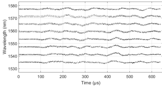
Fig. 3. 2 nd fiber (vertical) raw spectrogram recording with the BraggPulse .
