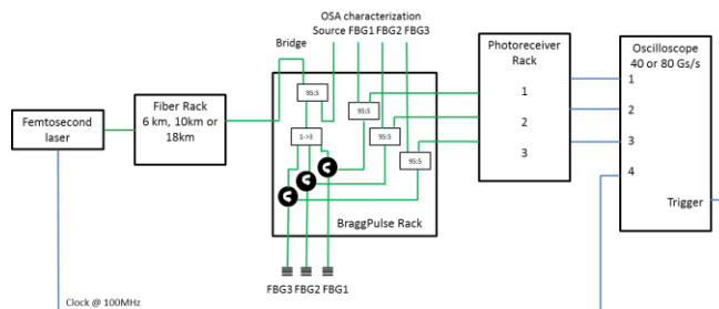
Fig. 1. Three FBG dynamic dispersive interrogator systems sharing the same wavelength to time conversion stage ( BraggPulse system).
