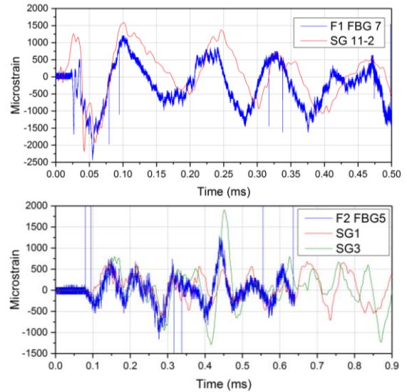
Fig. 4. Electrical strain gauges vs. FBG a) inside the cylinder and near the detonators b) outside the cylinder in the middle of height.
