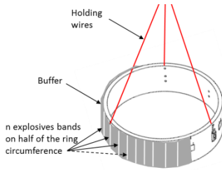
Fig. 2. Sketch of an experimental setup in the case of a ring sample.
