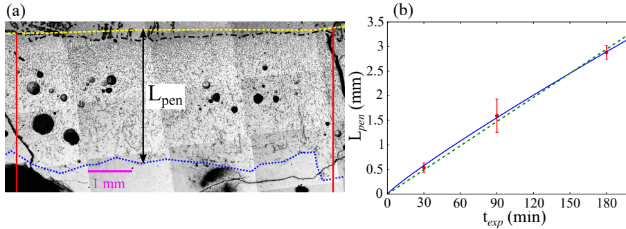
Figure 8: (a) BSE composite image representing the penetration length analyses procedure. (b) Average penetration length of molten steel dissolution attack as function of the exposure time at T=1700 °C. Solid line corresponds to the fitting curve using Equation 1. "Dash" line corresponds to a linear fit. Error bars represent the standard deviation.
