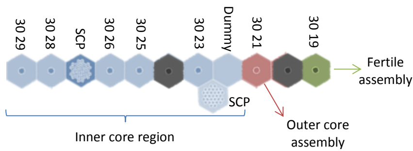
Figure 7. Irradiation column description in T1 and T2
