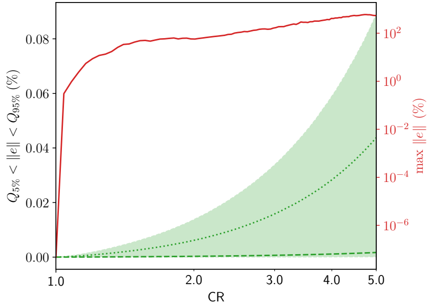
(a) Range within 5% and 95% quantiles (left) and its maximum value (right) by DCT on the whole dataset.
