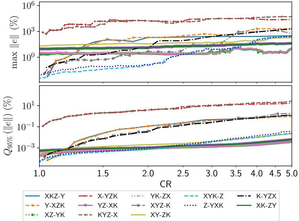
Figure 4: Maximum relative error and the 95% quantile computed after HT and progressive truncation on the different matrixization options.
