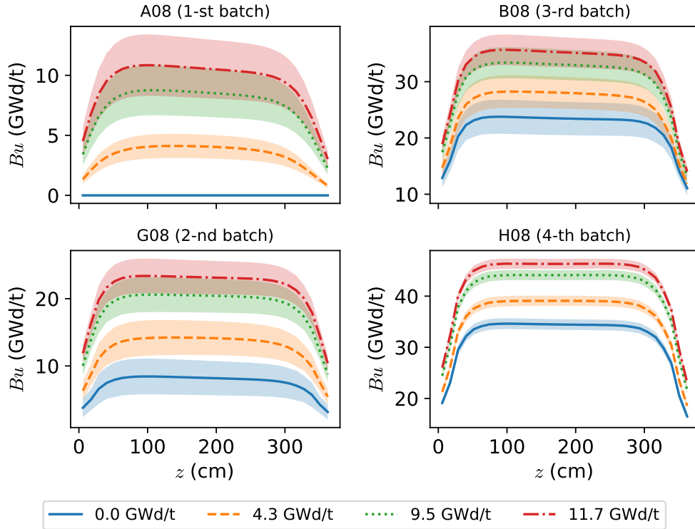
Figure 2: Axial distributions of the average pin burnup for four different FAs, selected at different core cycle burnup.
