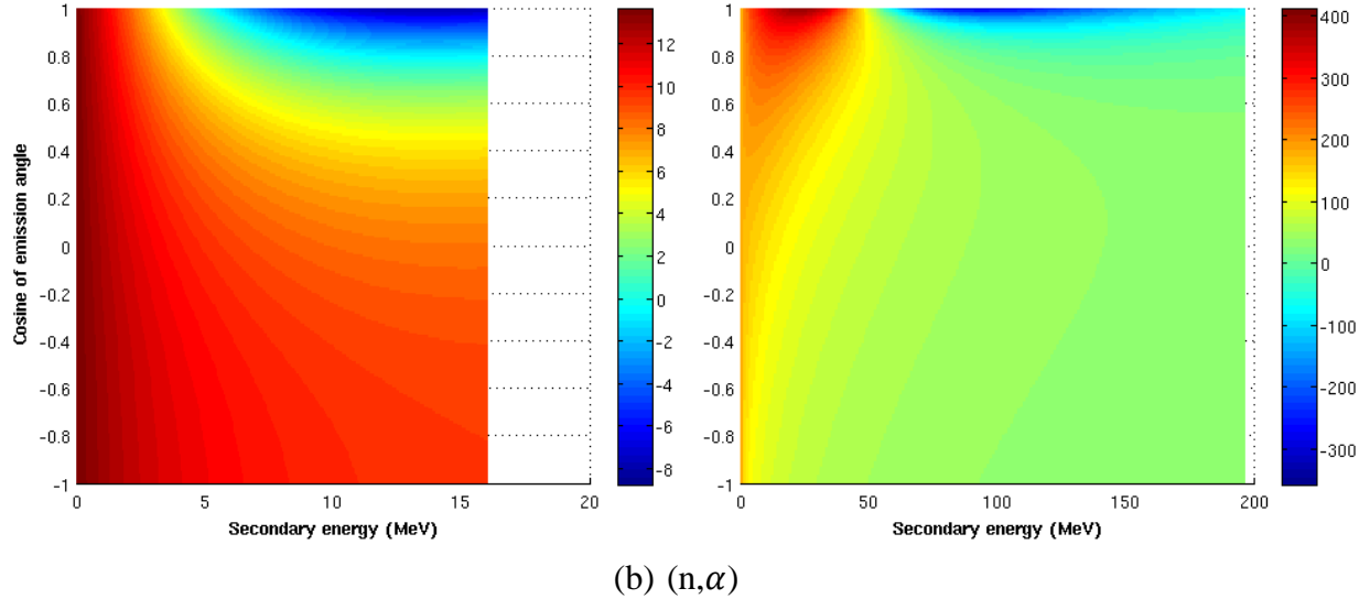
Figure 11. Difference of relativistic and classic mechanical NRT-DPA for 20 MeV (left) and 200 MeV (right) incident neutrons for proton emission reaction (a) and \alpha emission reaction (b) of ^{56}\text{Fe}
