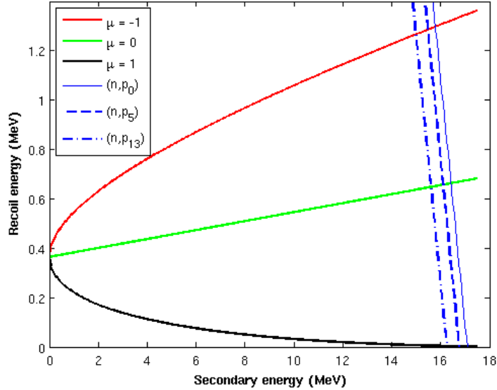
Figure 7. Recoil energy within special relativity versus secondary energy obtained with Eq. (9) ( \mu = -1, 0, 1 ) and Eq. (12) (blue lines) for 20 MeV neutron discrete (n,p) reactions of ^{56}\text{Fe}
