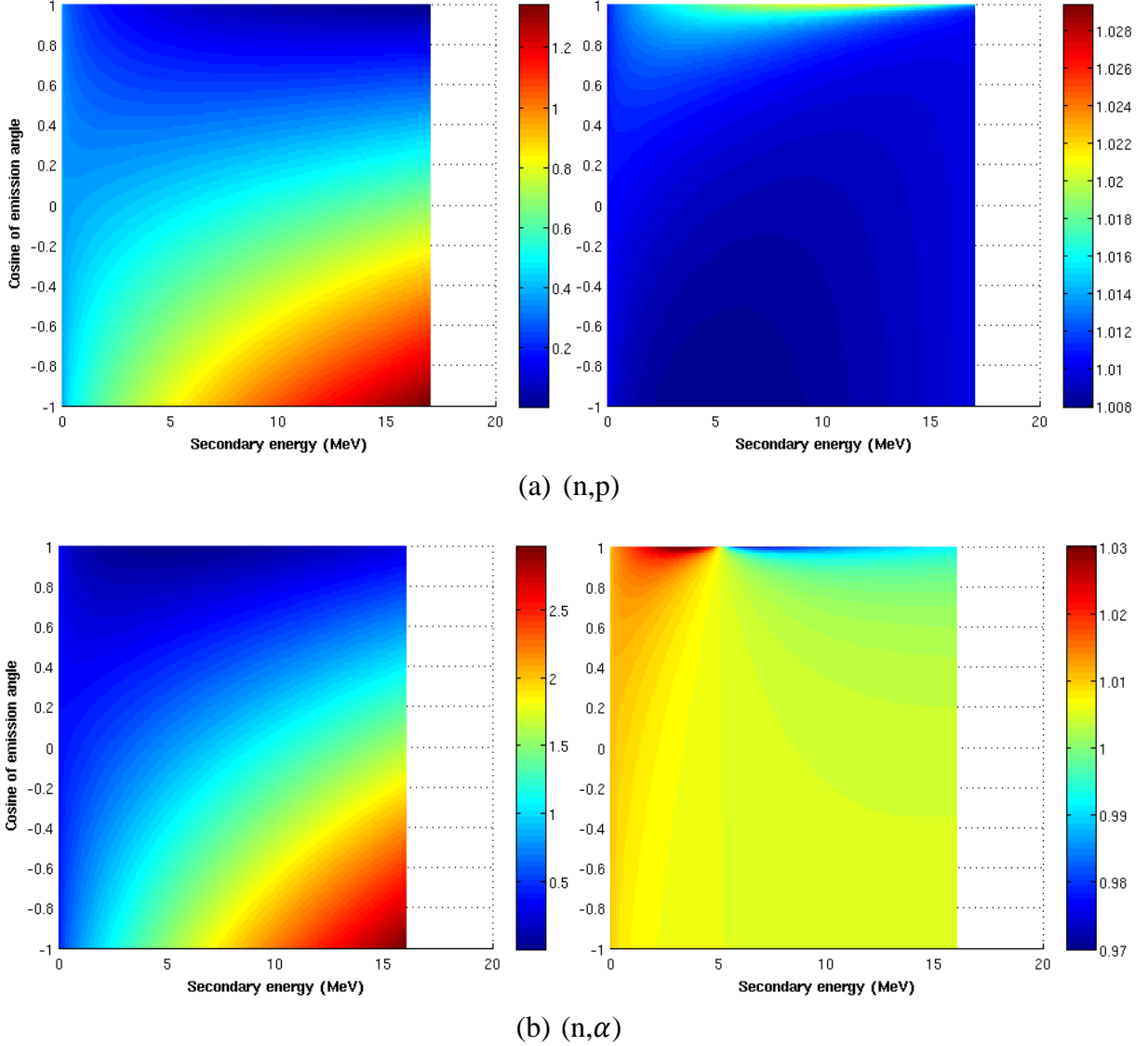
Figure 3. Recoil energy within special relativity (left, in MeV) for 20 MeV neutron-induced proton emission reaction (a) and \alpha emission reaction (b) of ^{56}\text{Fe} and the ratio of relativistic to classic mechanical results for all nuclei (right)
