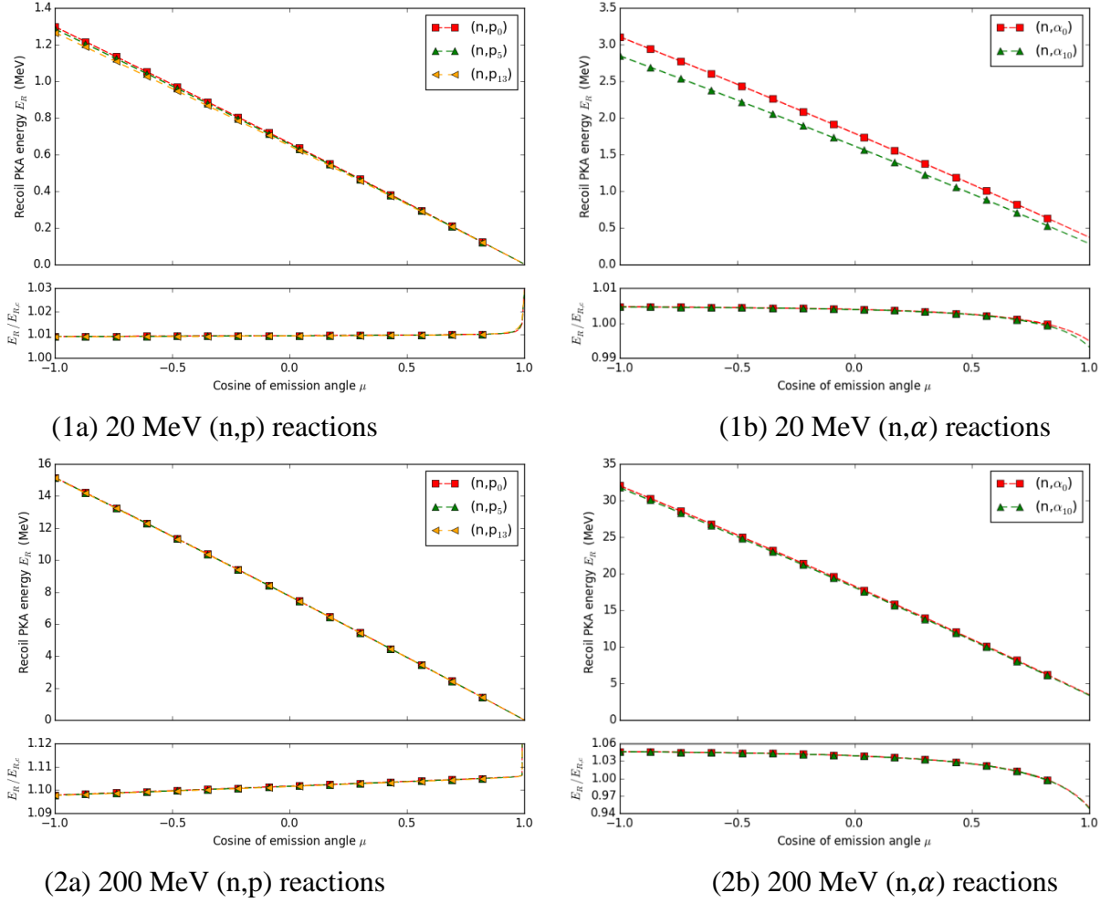
Figure 8. Recoil energy versus \mu for relativistic kinematics and the corresponding relativistic corrections for 20 MeV and 200 MeV neutron-induced discrete p and \alpha emissions of ^{56}\text{Fe}
