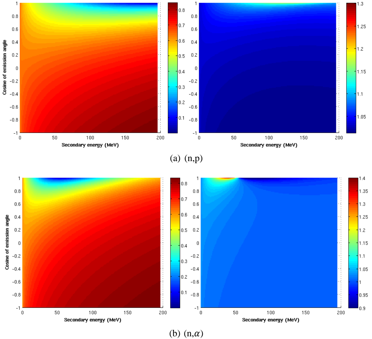
Figure 10. Damage energy within special relativity (left, in MeV) and the ratio of relativistic to classic mechanical results (right) for proton emission reaction (a) and \alpha emission reaction (b) of ^{56}\text{Fe} with 200 MeV incident neutrons
