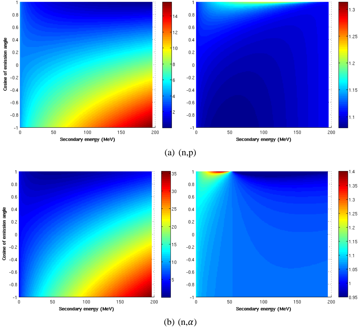
Figure 4. Recoil energy within special relativity (left, in MeV) for a 200 MeV neutron-induced proton emission reaction (a), and \alpha emission reaction (b) of ^{56}\text{Fe} and the ratio of relativistic to classic mechanical results for all nuclei (right)
