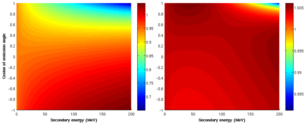
Figure 9. Damage energy within special relativity (left, in MeV) for 200 MeV \alpha induced ( \alpha ,n) reaction of ^{56}\text{Fe} and the corresponding ratio of relativistic to classic mechanical results (right)
