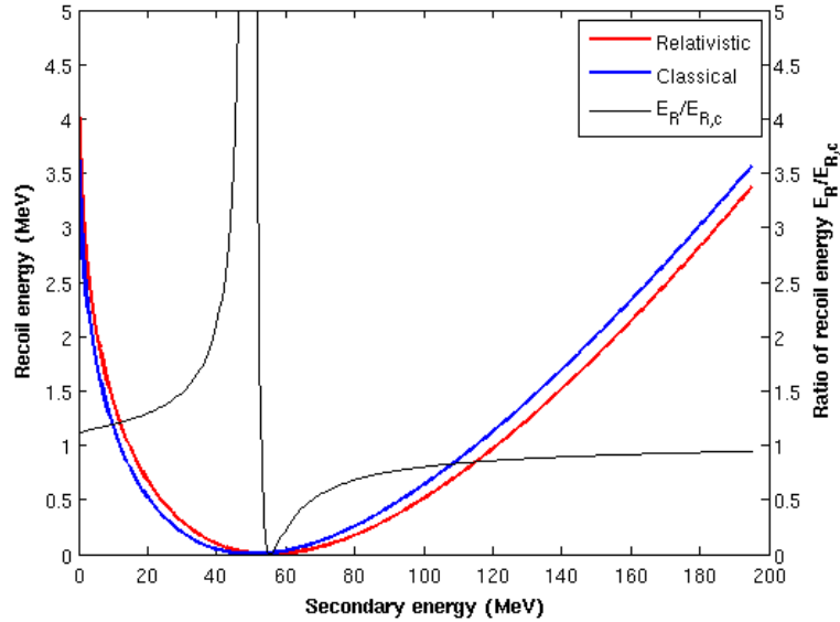
Figure 6. Recoil energies within special relativity and classical mechanics versus secondary energy for the 200 MeV neutron-induced (n, \alpha ) reaction with ^{56}\text{Fe} at \mu = 1
