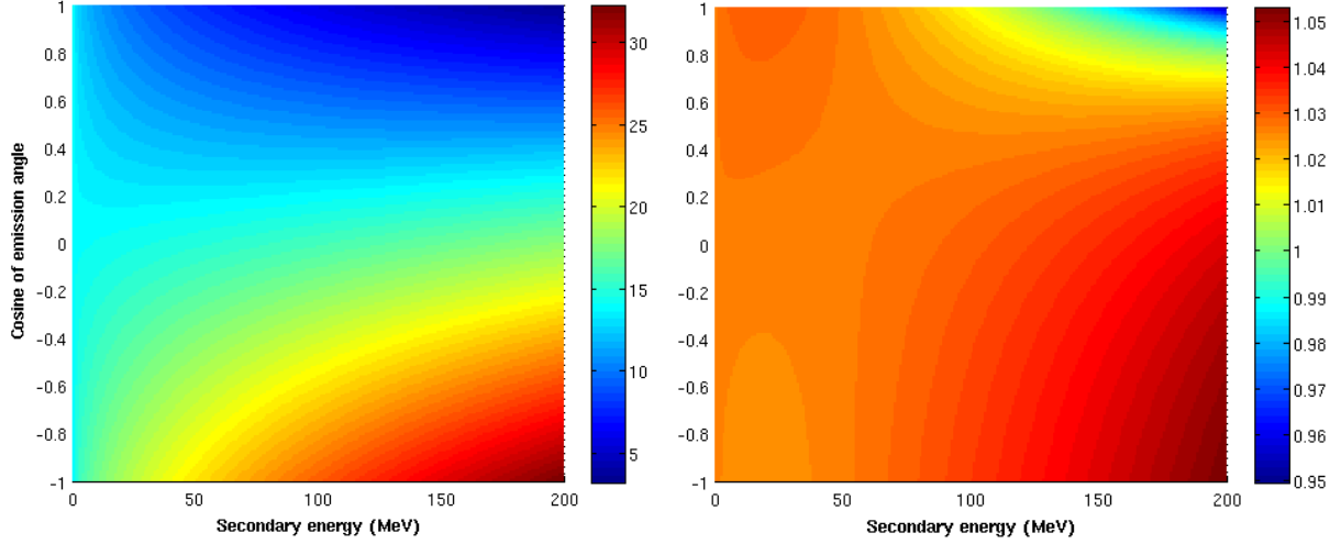
Figure 5. Recoil energy within special relativity (left, in MeV) and 200 MeV \alpha induced ( \alpha ,n) reaction of ^{56}\text{Fe} and the ratio of relativistic to classic mechanical results for all nuclei (right)
