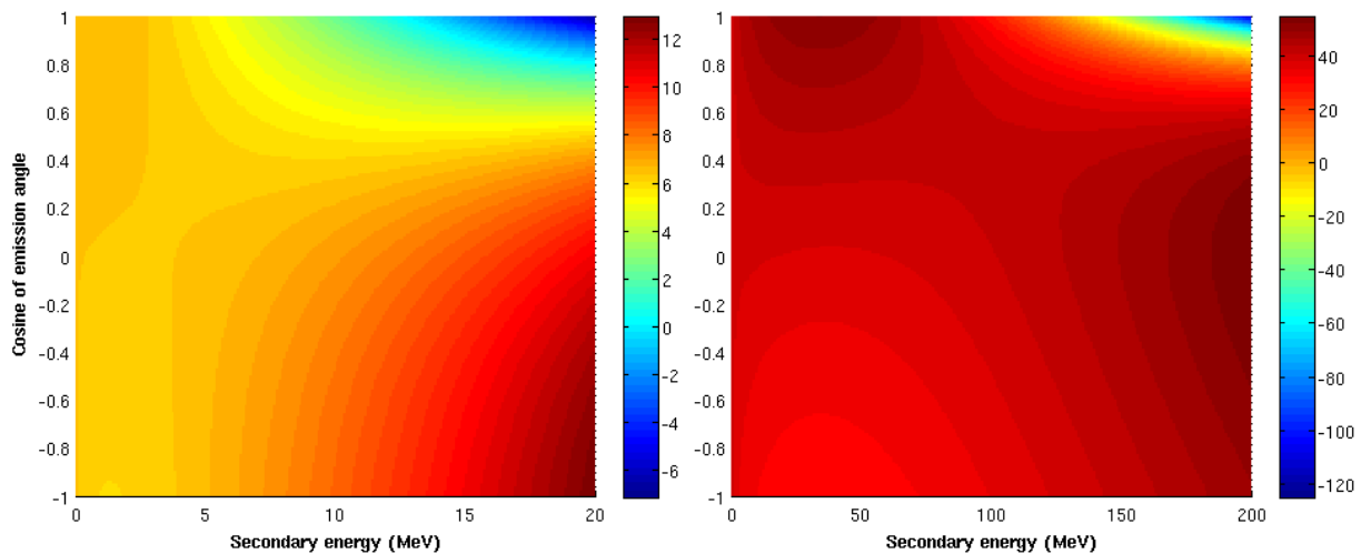
Figure 12. Difference of relativistic and classic mechanical NRT-DPA for 20 MeV (left) and 200 MeV (right) \alpha induced ( \alpha ,n) reaction of ^{56}\text{Fe}
