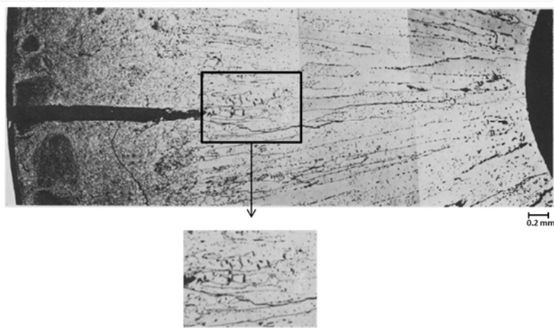
Figure 5 – Crack healing by production and migration of lenticular pore [17]
