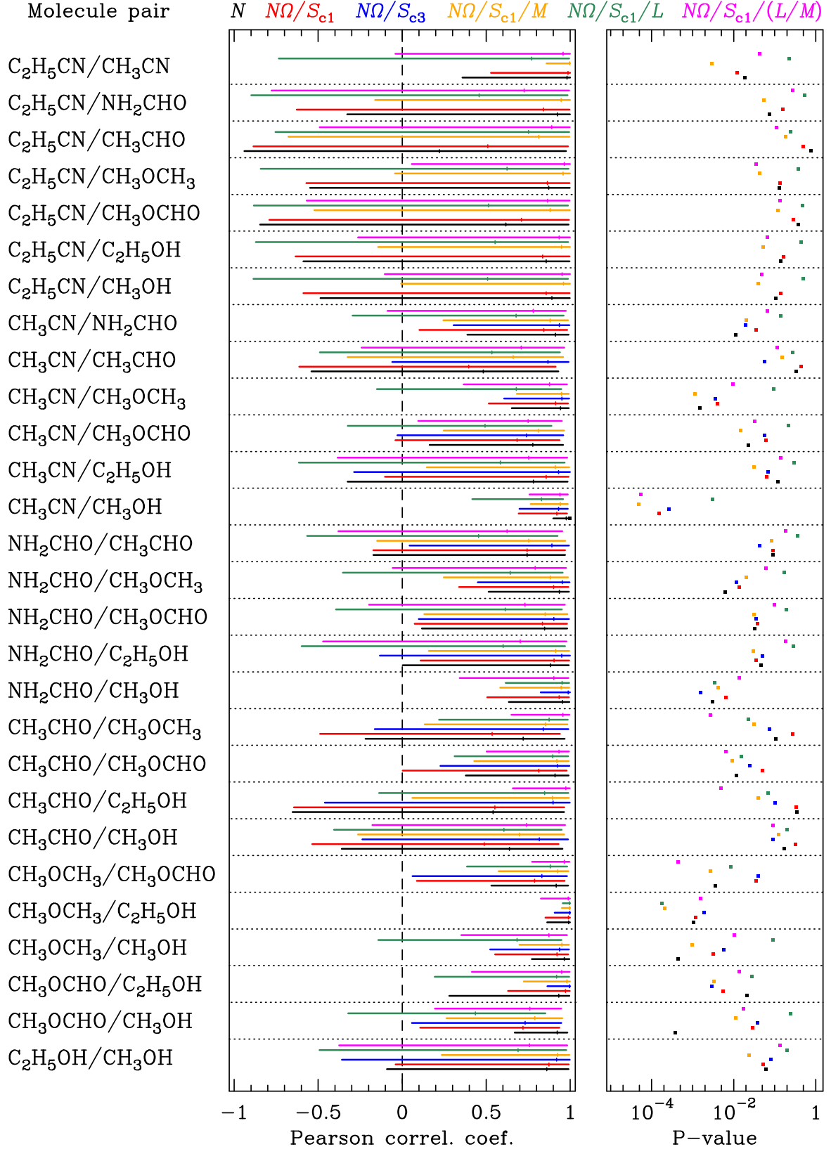
Fig. 7. Pearson correlation coefficients with 95% confidence interval (left) and P -value (right) for various pairs of COMs for the CALYPSO source sample. The P -value is the probability of observing a correlation plot under the null hypothesis of no correlation. These parameters were derived from the plots shown in Figs. H.1–H.6. The colors indicate the variables used to evaluate the degree of correlation between molecules: column density (black), column density multiplied by the solid angle \Omega of the COM emission and divided by either the 1.3 mm continuum peak flux density or the 1.3 mm continuum flux density integrated over the size of the COM emission, S_{c1} (red), column density multiplied by the solid angle of the COM emission and divided by the 3 mm continuum peak flux density (blue), column density multiplied by \Omega/S_{c1} and divided by the envelope mass (orange), column density multiplied by \Omega/S_{c1} and divided by the internal luminosity (green), column density multiplied by \Omega/S_{c1} and divided by the ratio of internal luminosity to envelope mass (magenta).
