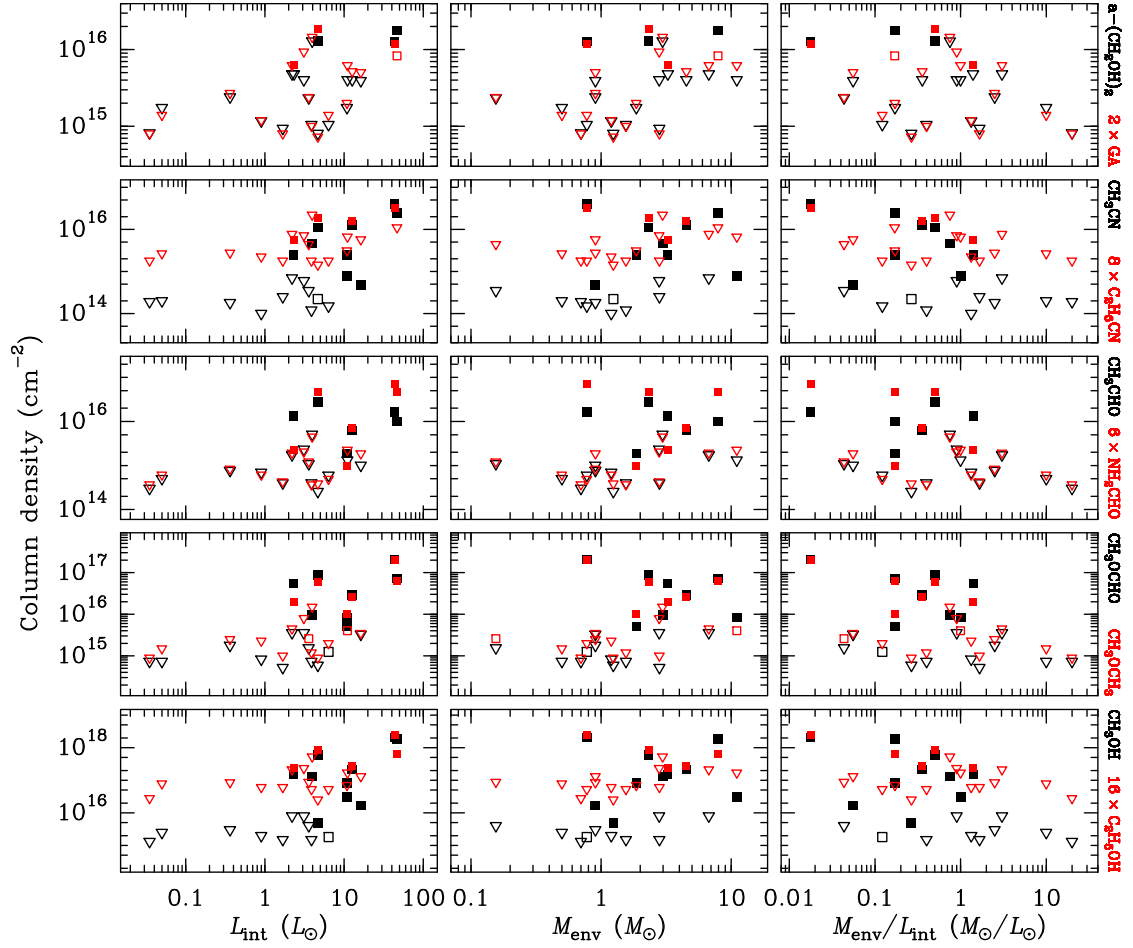
Fig. I.1. Column densities of ten complex organic molecules as a function of internal luminosity, envelope mass, and ratio of envelope mass to internal luminosity. The column densities of some molecules were multiplied by a scaling factor as indicated on the right. Filled and open squares represent robust and tentative detections, respectively, while open triangles show upper limits. GA stands for glycolaldehyde, \text{CH}_2(\text{OH})\text{CHO} .
