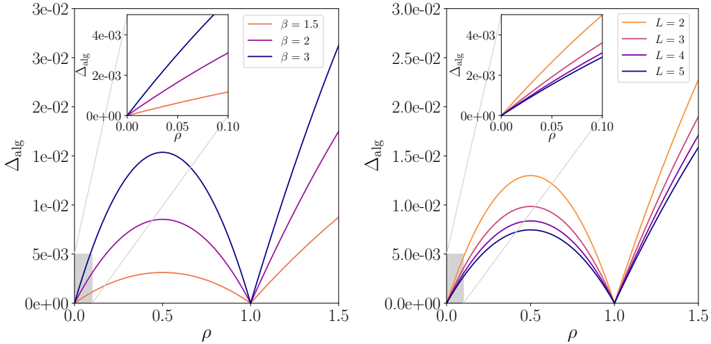
Figure 6: Algorithmic gap \Delta_{\text{alg}} = \alpha_{\text{alg}} - \alpha_{\text{T}} for small \rho and linear activation, as a function of (left) the compression \beta \equiv \beta_l for fixed depth L = 4 and of (right) depth for a fixed compression \beta = 2 .
