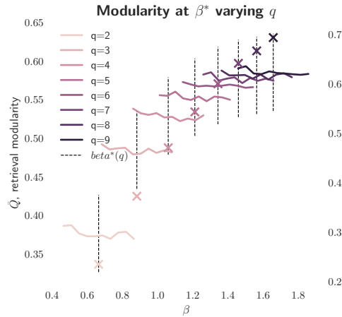
Fig. S.13: Using the method recommended by Zhang and Moore to select the appropriate value of q for the American NCAA Div-IA College Football Network [15, 10]. Each colored line corresponds to running modbp for a given value of q across a window of \beta around \beta^*(q) (shown by black dashed line). Using this method would suggest an appropriate q \in [6 - 8] depending on the threshold selected. We note that here, we do not collapse community labels as described in Section 2.3; for each run a single fixed value of q is used as well as the default resolution ( \gamma = 1 ).
