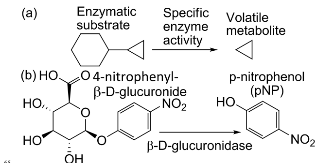
Fig. 1 (a) Enzymatic hydrolysis of enzymatic substrate releasing volatile metabolite. (b) Hydrolysis of 4-nitrophenyl-β-D-glucuronide (pNPG) releasing colored volatile p-nitrophenol.
