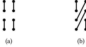
Figure 8: Different types of diagrams of indices appearing in \langle U^4 \rangle_0
