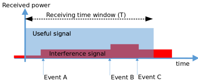
Fig. 3. Calculating SINR in a receiving vehicle
