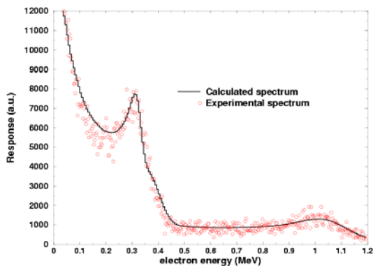
Fig. 3. Measured and calculated pulse height spectrum for Na22.
