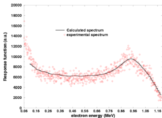
Fig. 4. Measured and calculated pulse height spectrum for Co60.
