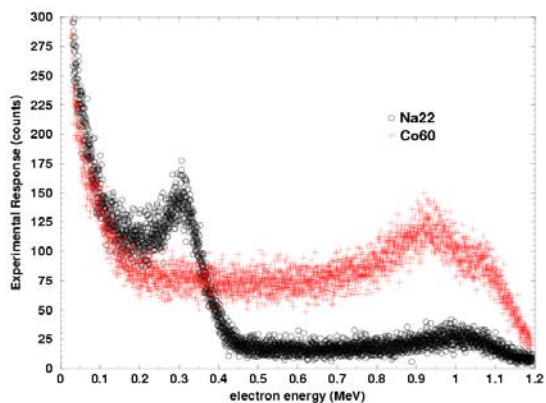
Fig. 1. Experimental Pulse Height Distributions.
