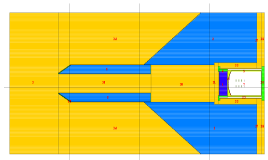
Fig. 2. Experimental set-up simulated by MCNPX2.5e.
