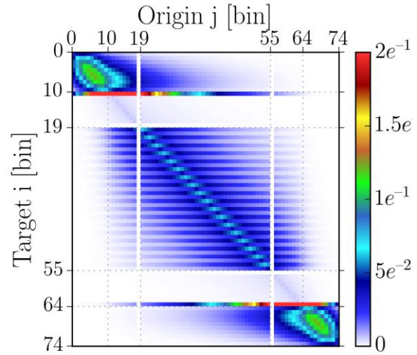
Figure 7: « delayed-to-prompt » fission matrix
