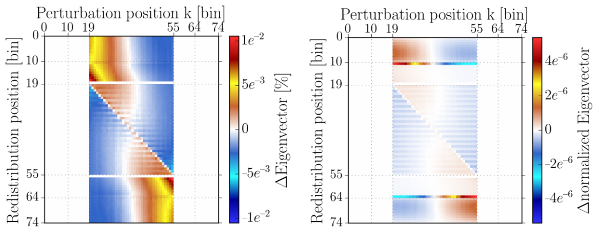
Figure 15: Eigenvector matrix redistribution due to local Na perturbation in bin 34. Left: perturbation on the eigenvector/bin (in %) – Right: normalized perturbation
