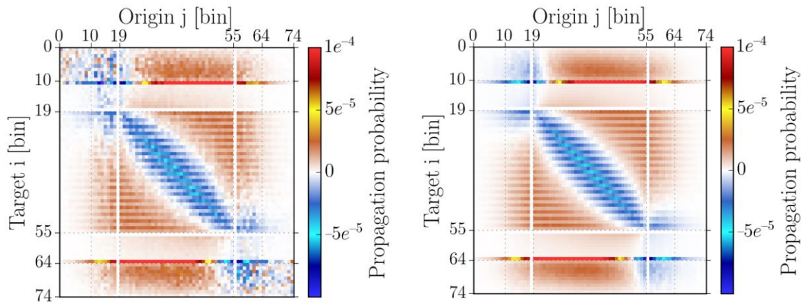
Figure 12: " vp \rightarrow \chi p " discrepancy between two states by independant Monte Carlo approach (left) and correlated sampling (right)
