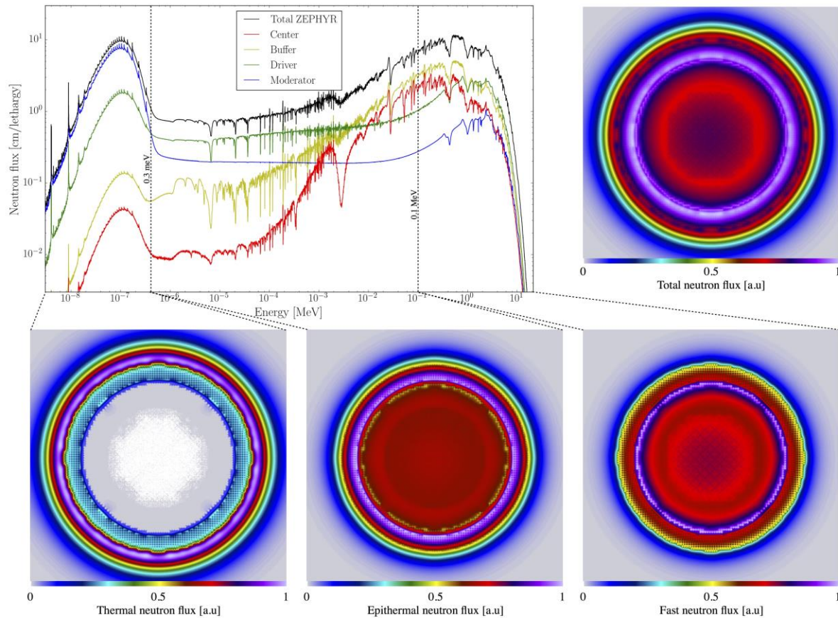
Figure 3: Neutron spectra in the different areas of ZEPHYR (upper left) together with the neutron flux maps calculated with the Serpent2 code: total flux (upper-right), and thermal/epithermal/fast flux (bottom)
