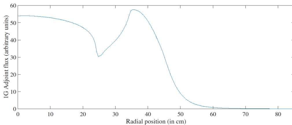
Figure 4: Radial representation of the 1G adjoint flux in the ZEPHYR fast/thermal coupled configuration
