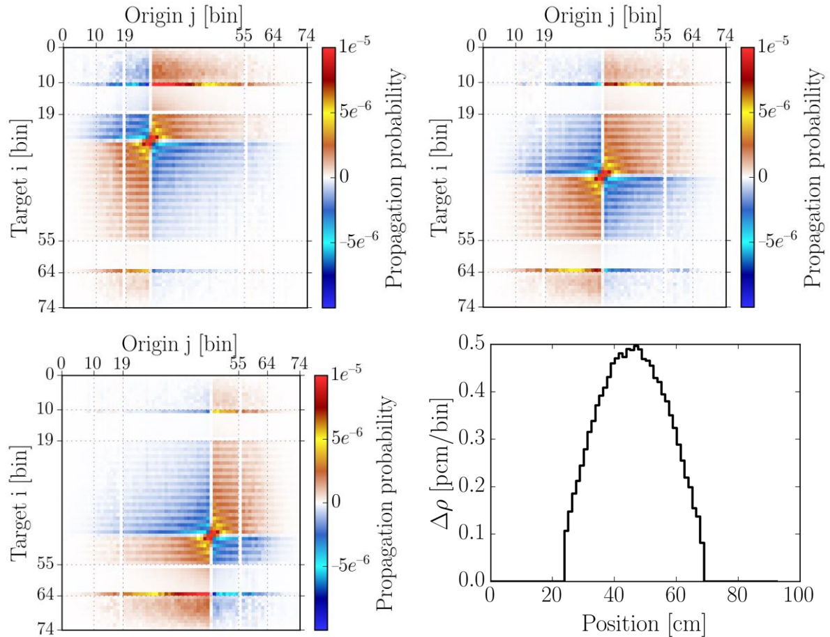
Figure 14: evolution of the fission matrix as the density perturbation crosses the geometry. The sensitivity profile of the reactivity per perturbed bin is also reproduced (lower right)
