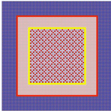
Figure 5a: squared 2D representation of the ZEPHYR optimized fast/thermal coupled configuration
