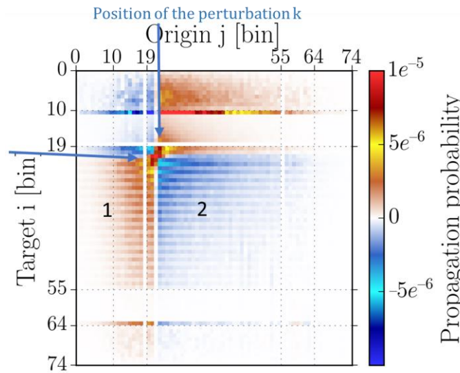
Figure 13: local impact of a 1% perturbation in the sodium density on the fission probabilities
