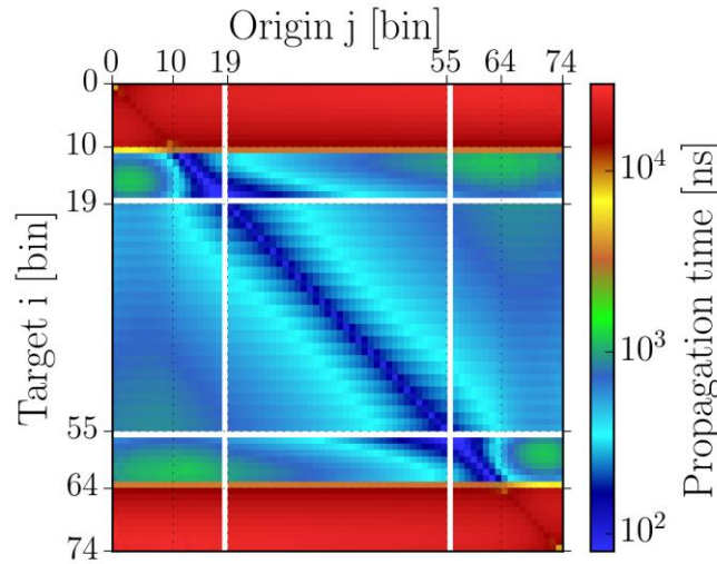
Figure 11: "prompt to prompt" time operator matrix
