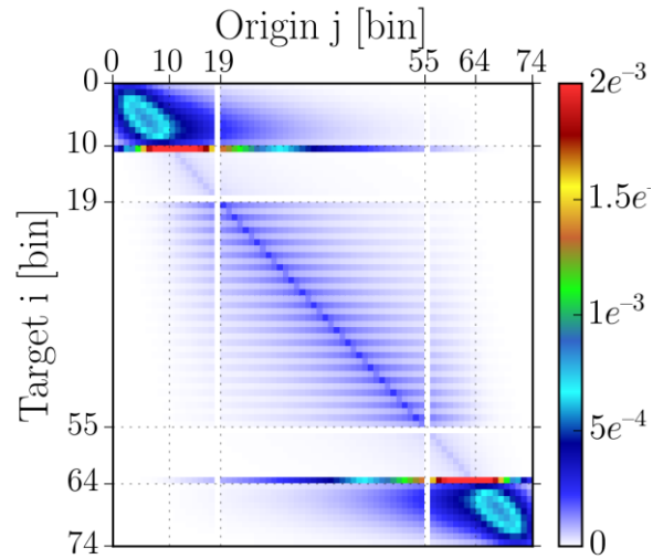
Figure 10 : « delayed-to-delayed » fission matrix
