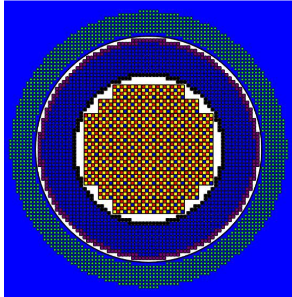
Figure 2: X-Y representation of the TRIPOLI4® modelling of the Fast/Thermal optimized configuration
