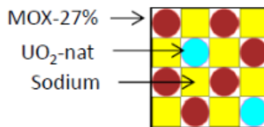
Figure 1: ZONA1 MOX unit cell
