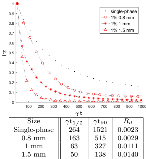
Fig. 17: Influence of the particle size on the intra-vortex mixing I_{rz} in TVF regime ( Re=100 , \lambda = 2.25e ) for particle concentration of 1%. Mixing times and initial decay rate are reported in the table.
