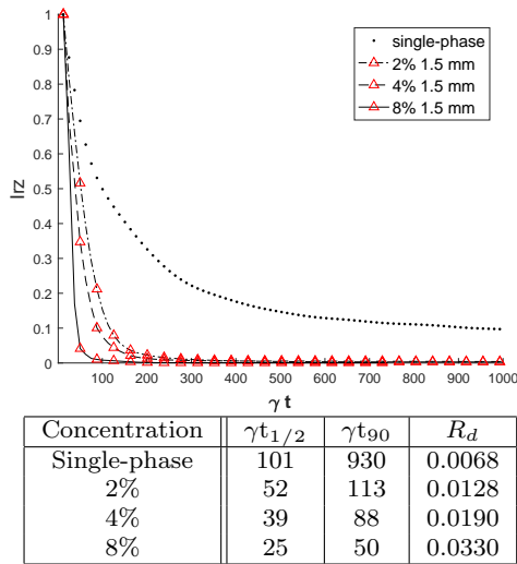
Fig. 14: Influence of the particle concentration on the intra-vortex mixing I_{rz} in TVF regime for particle size of 1.5 mm ( Re=100 , \lambda = 2.25e ). Mixing times and initial decay rate are reported in the table.
