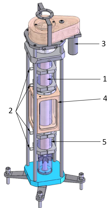
Fig. 1: Experimental device: 1. Rotor; 2. Sampling ports; 3. Motor; 4. Visualization box; 5. Stator.
