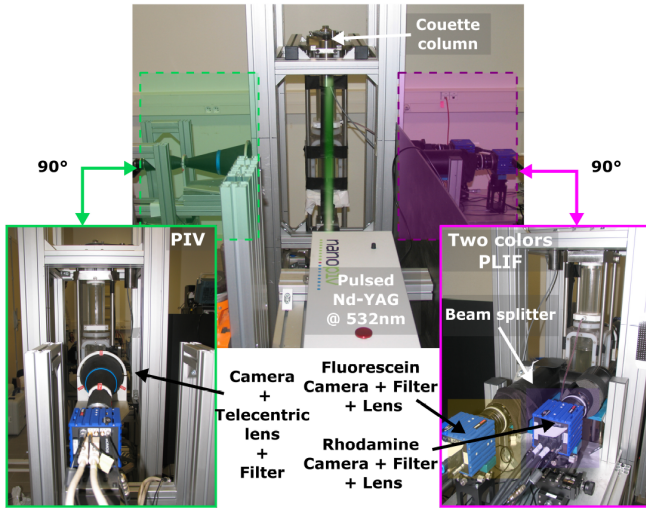
Fig. 7: Experimental devices for the coupled PIV/PLIF measurements.
