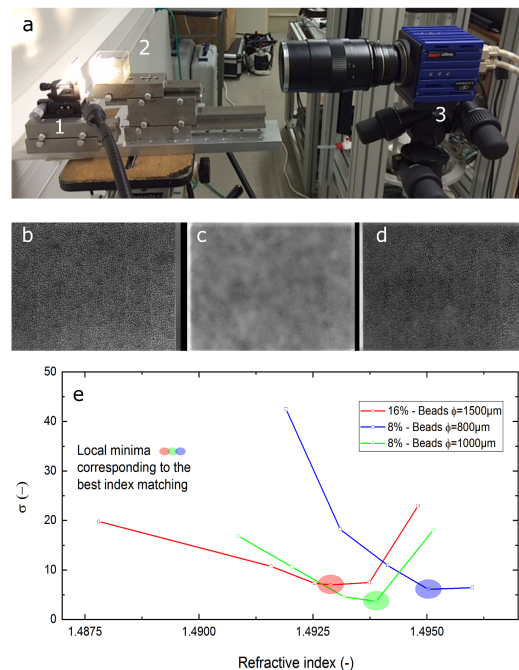
Fig. 3: (a) Experimental setup used to match refractive index and density - Images of the random pattern used for PIV correlation in the tank for a perfect matching (b), a lack of matching (c) and a partial matching (d) - (e) The best mixture of fluids is achieved for the local minimum of each curve.
