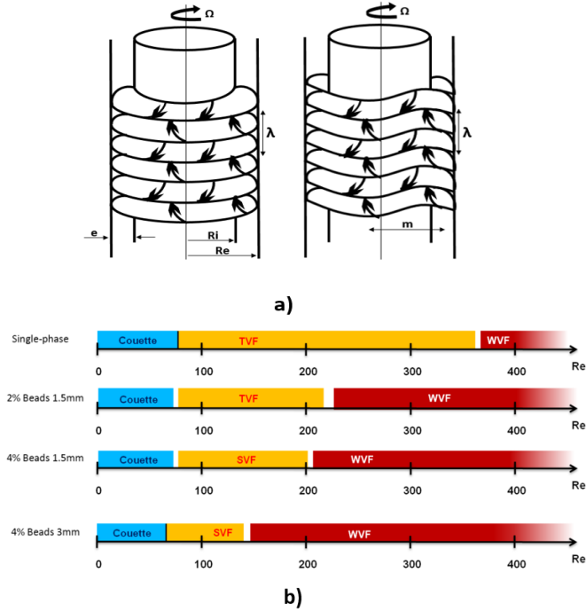
Fig. 2: a): Visualization of the flow regimes by increasing the rotation rate (TVF (left), WVF (right)), and their corresponding axial wavelengths \lambda . b) Particles effect on the flow transition. From top to bottom: single-phase flow configuration, R_i/R_e = 0.687 and two-phase flows with increasing bead size and concentrations, R_i/R_e = 0.687 .
