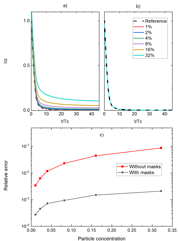
Fig. 11: (a) I_{rz} as a function of time without dynamic masks correction, (b) I_{rz} as a function of time with dynamic masks correction, (c) Evolution of relative error with increasing volume fraction of particles.
