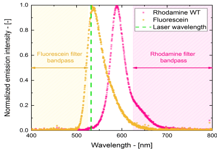
Fig. 5: Emission spectrum of fluorescein and rhodamine WT
