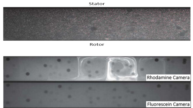
Fig. 4: Top: PIV image obtained in the presence of 1.5 mm beads, the image is cropped to fit with the region of interest and rotated by 90°. Bottom: Two simultaneous acquisitions of the PLIF rhodamine WT image (top) and the fluorescein image (bottom). Case of a 4% volume concentration of 1.5 mm beads in TVF regime ( Re = 90 ).
