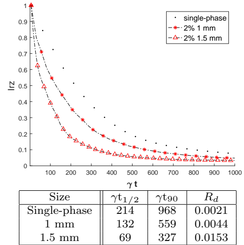
Fig. 18: Influence of the particle size on the intra-vortex mixing I_{rz} in WVF regime ( Re=600 , \lambda = 2e ) for particle concentration of 2%. Mixing times and initial decay rate are reported in the table.
