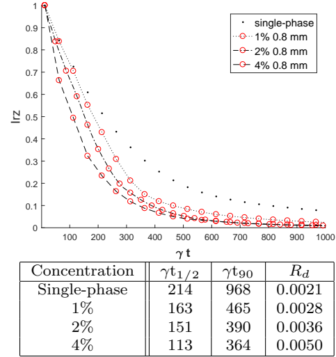
Fig. 15: Influence of the particle concentration on the intra-vortex mixing I_{rz} in WVF regime for particle size of 0.8mm ( Re=600 , \lambda = 2e ). Mixing times and initial decay rate are reported in the table.
