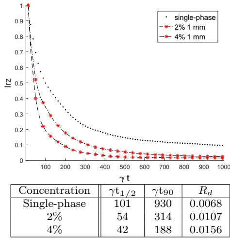
Fig. 13: Influence of the particle concentration on the intra-vortex mixing I_{rz} in TVF regime for particle size of 1mm ( Re=100 , \lambda = 2.25e ). Mixing times and initial decay rate are reported in the table.
