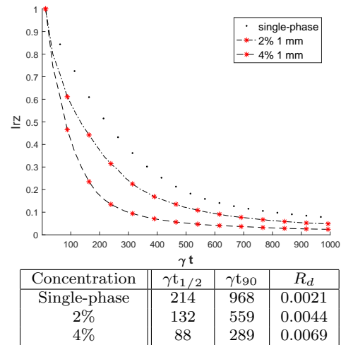
Fig. 16: Influence of the particle concentration on the intra-vortex mixing I_{rz} in WVF regime for particle size of 1 mm ( Re=600 , \lambda = 2e ). Mixing times and initial decay rate are reported in the table.
