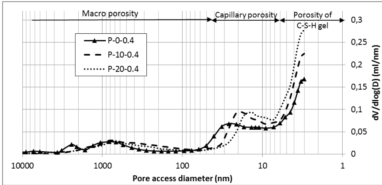
Fig. 4: Effect of SF addition on pore size distribution
