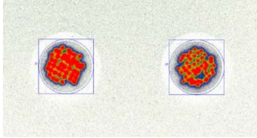
Fig 2: Homogeneity of two sources Cl-36 (left) and Sr-90 (right) showed by an exposure on autoradiographic screen.
