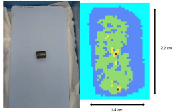
Fig 7: Graphite core deposited on a DA screen (left) and the homogeneity of C-14 (right)
