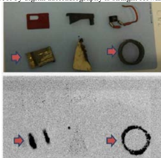
Fig. 5. Example of potential tritiated materials containing (red arrows) or not H-3 (black image on autoradiographic image).
