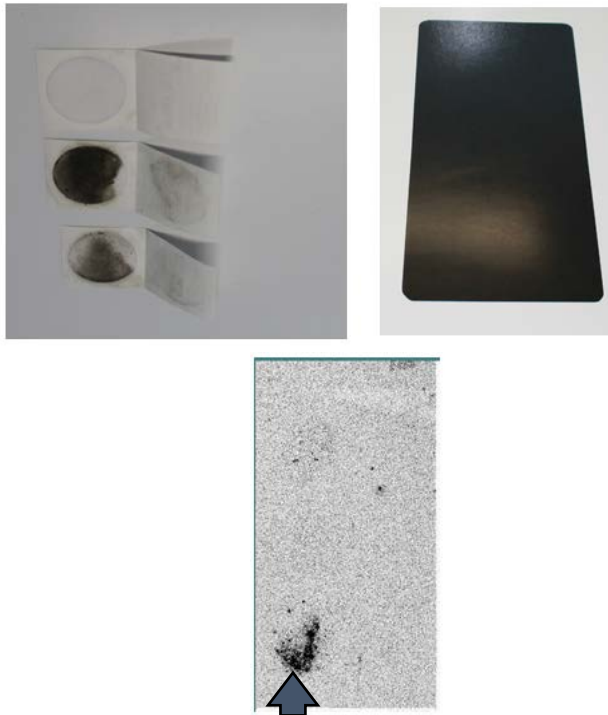
Fig 6: Example of the effect of three wipes on a DA screen (top the measurement with a screen deposited on the wipes, bottom the effect of the presence of uranium)
