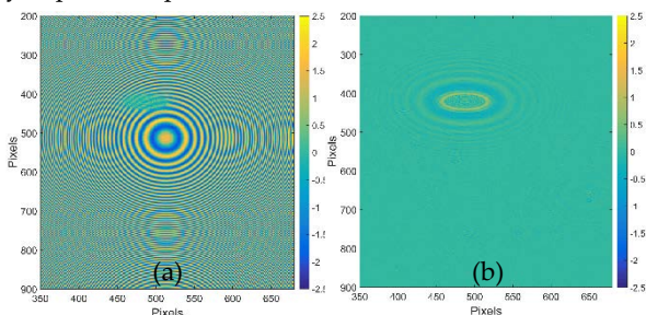
Figure 3: Imaginary part of the focused field by FrFT at z = 40mm with (a) supplementary FrFT phase (b) phase correction
