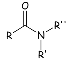
N,N dialkylamide
