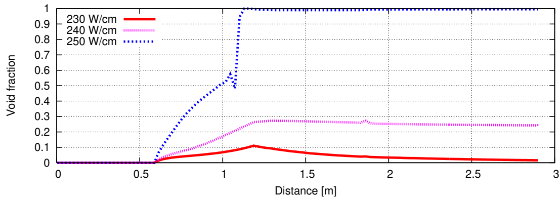
Figure 5: Void fraction inside the hot channel.
