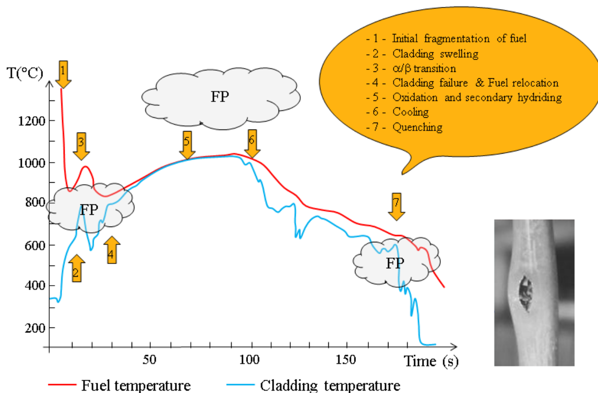
Figure 1: Different phases of a typical LOCA sequence.
