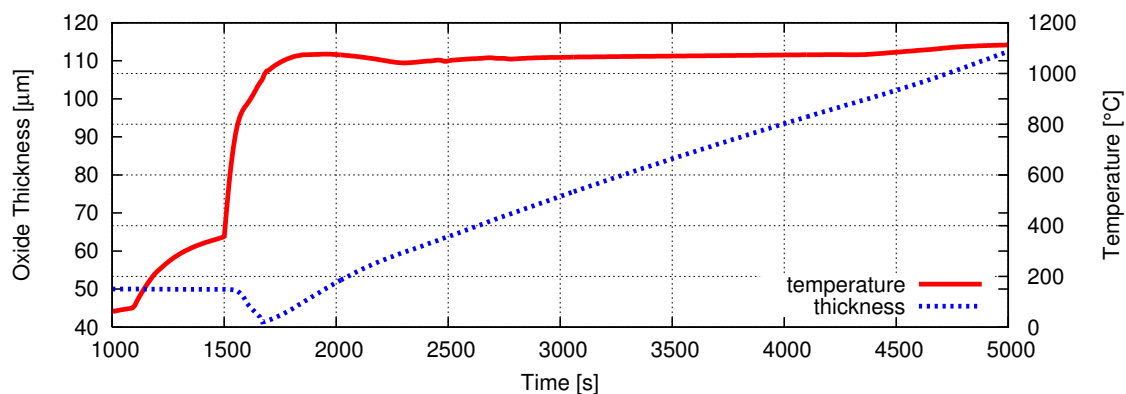
Figure 9: External cladding temperature and thickness oxidation in the center of the fuel
