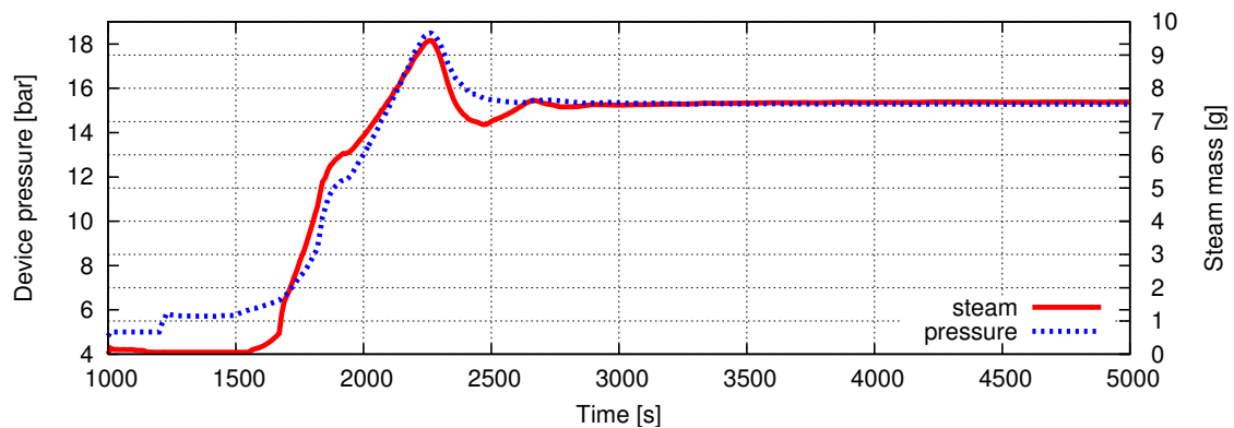
Figure 8: Pressure and steam mass inside the hot channel.
