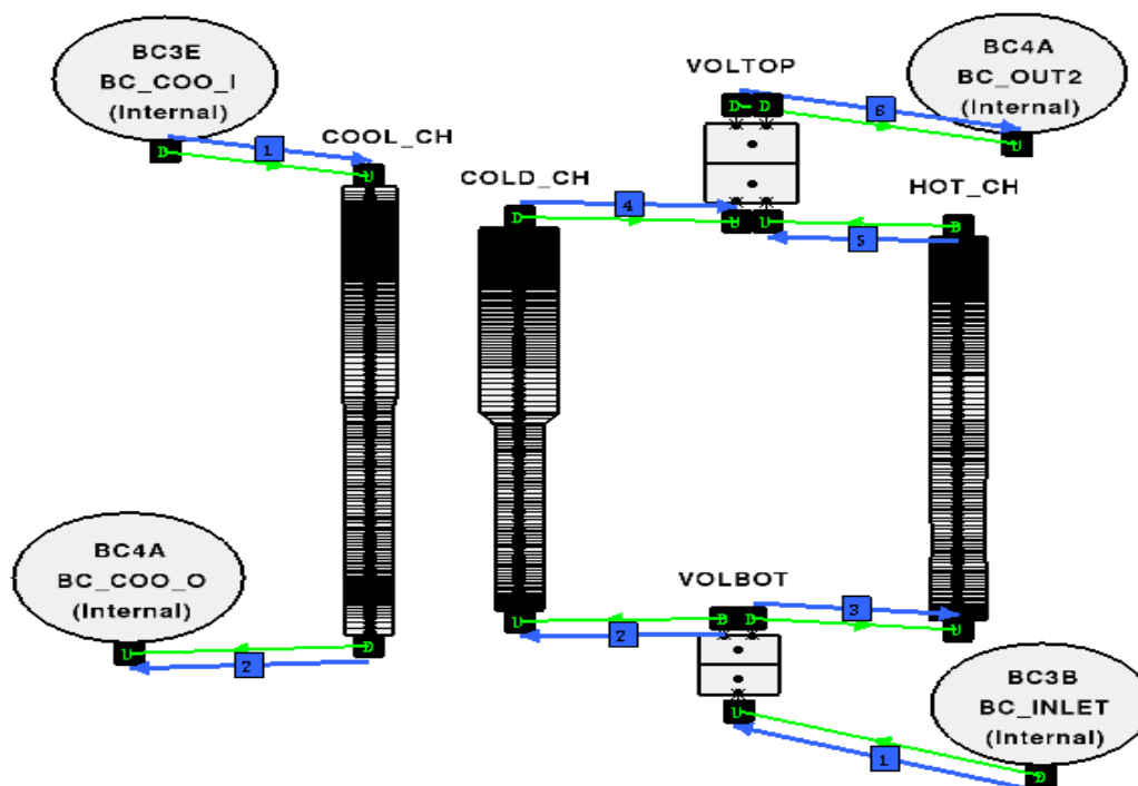
Figure 3: LORELEI modeling with CATHARE.
