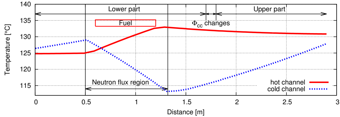
Figure 4: Liquid temperature along the hot and cold channels.
