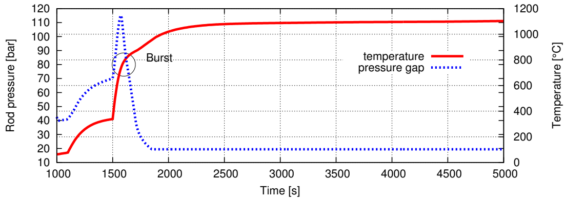
Figure 7: Clad temperature and pressure inside the fuel gap.
