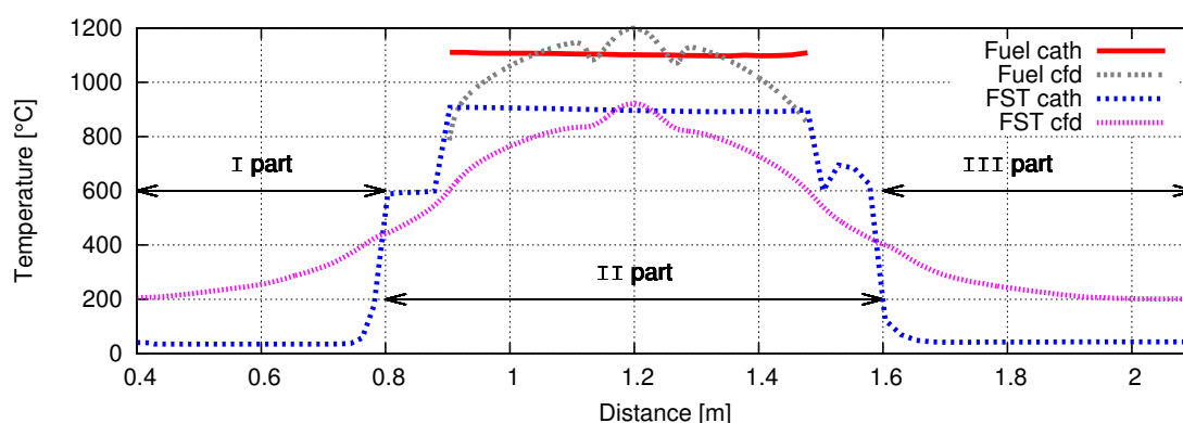
Figure 6: Wall temperature calculated with CATHARE and CFD.
