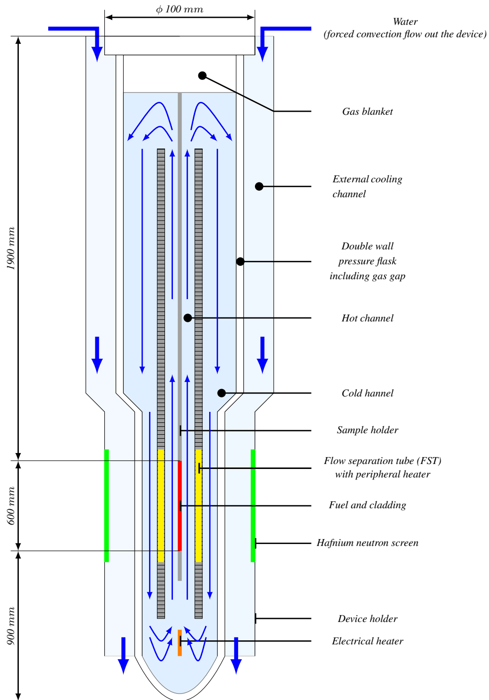
Figure 2: Simplified layout of LORELEI.
