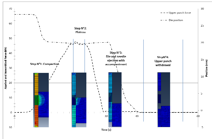
Fig 9: Von-Mises stress during each shaping cycle steps
