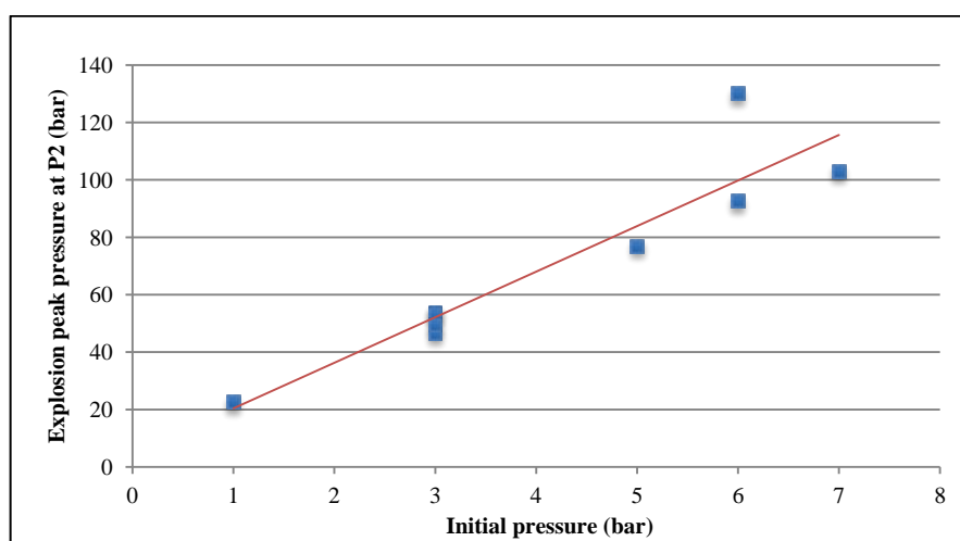
Figure 3 : explosion peak pressure (P2 sensor) vs initial pressure
