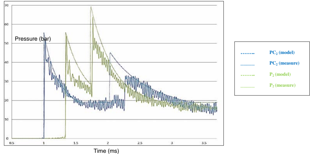
Figure 4 : example of a model-measurement comparison (experiment n°2a)
