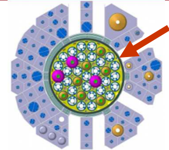
In JHR reflector on a displacement system
